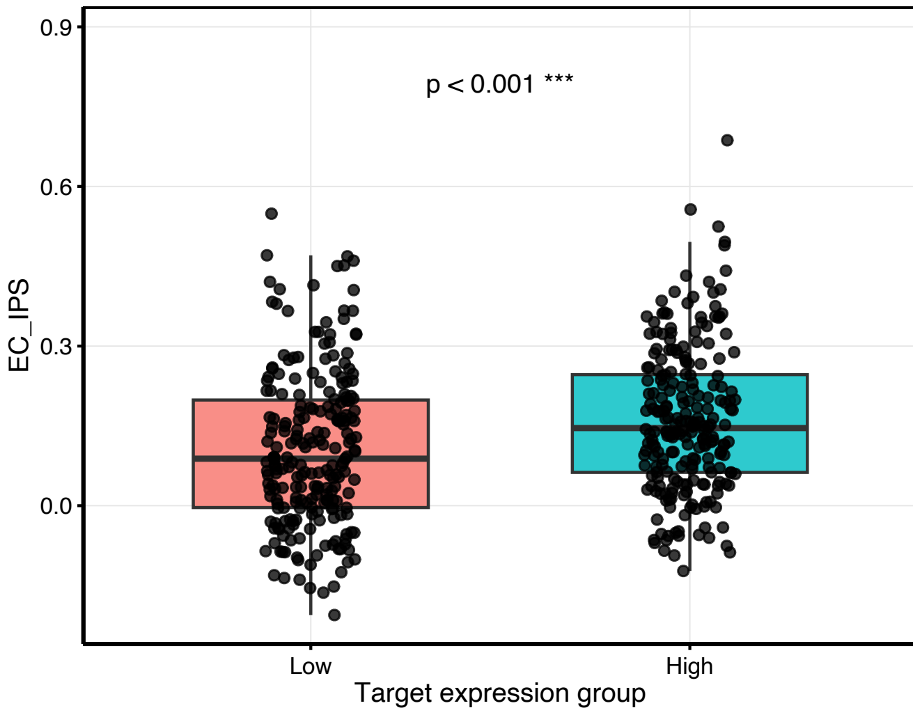
TCGA_COAD_01A_ATF3_ips EC_IPS by Target expression group
