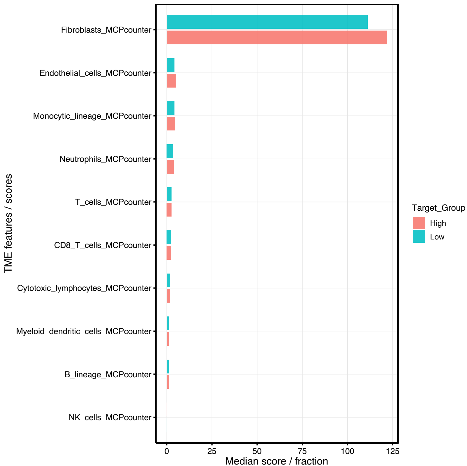
TCGA_COAD_01A_ATF3_mcpcounter cell fractions by group
