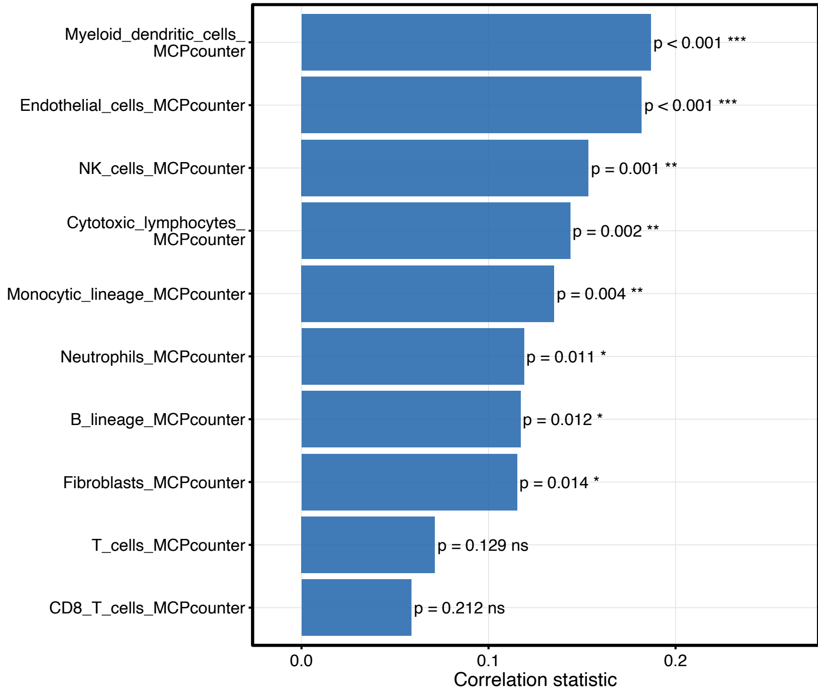
TCGA_COAD_01A_ATF3_mcpcounter correlation with target gene
