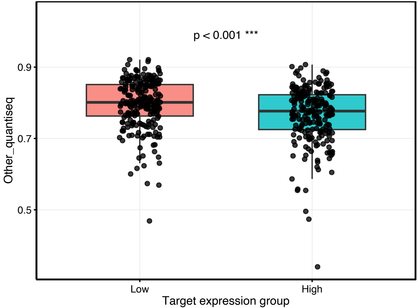
TCGA_COAD_01A_ATF3_quantiseq Other_quantiseq by Target expression group
