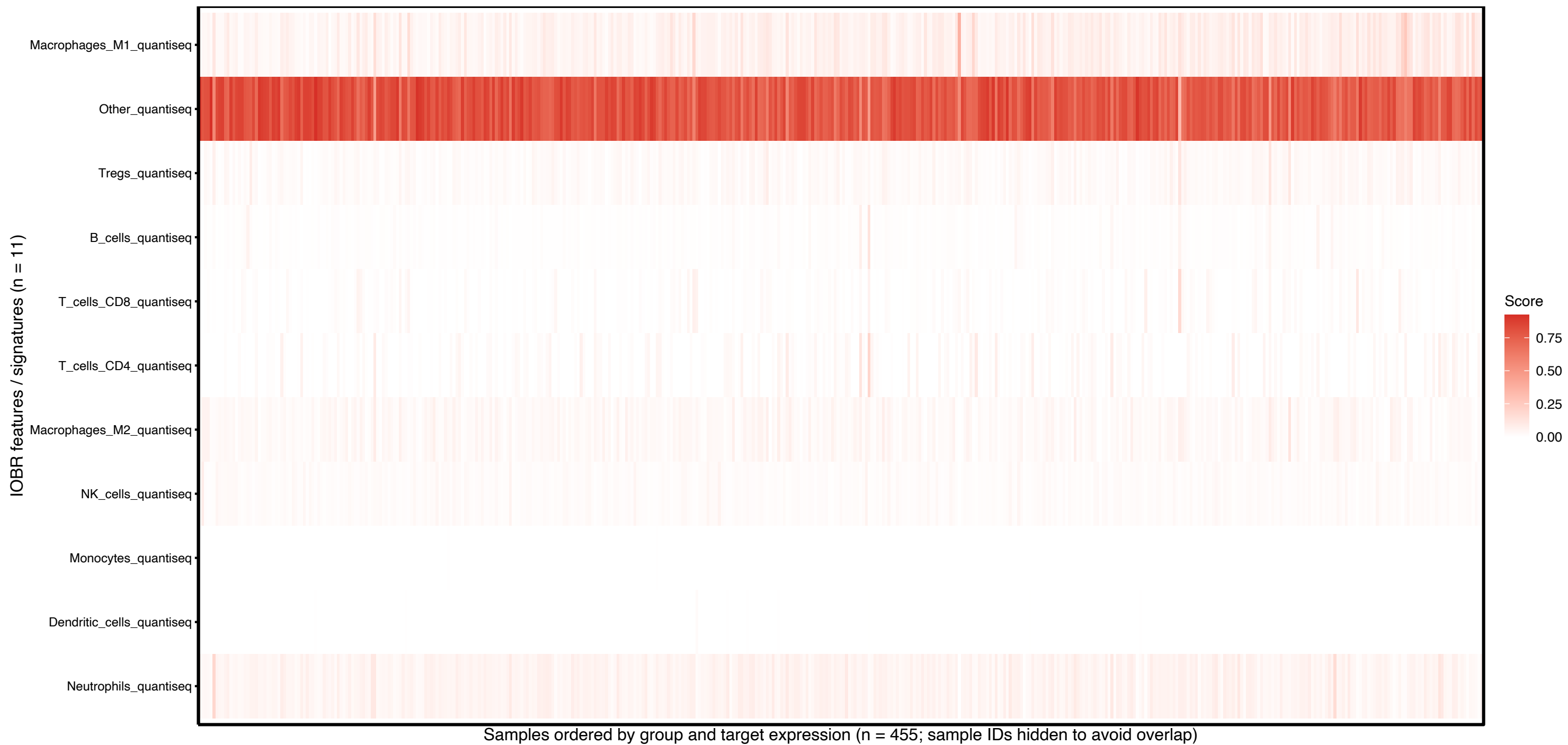
TCGA_COAD_01A_ATF3_quantiseq all IOBR features heatmap
