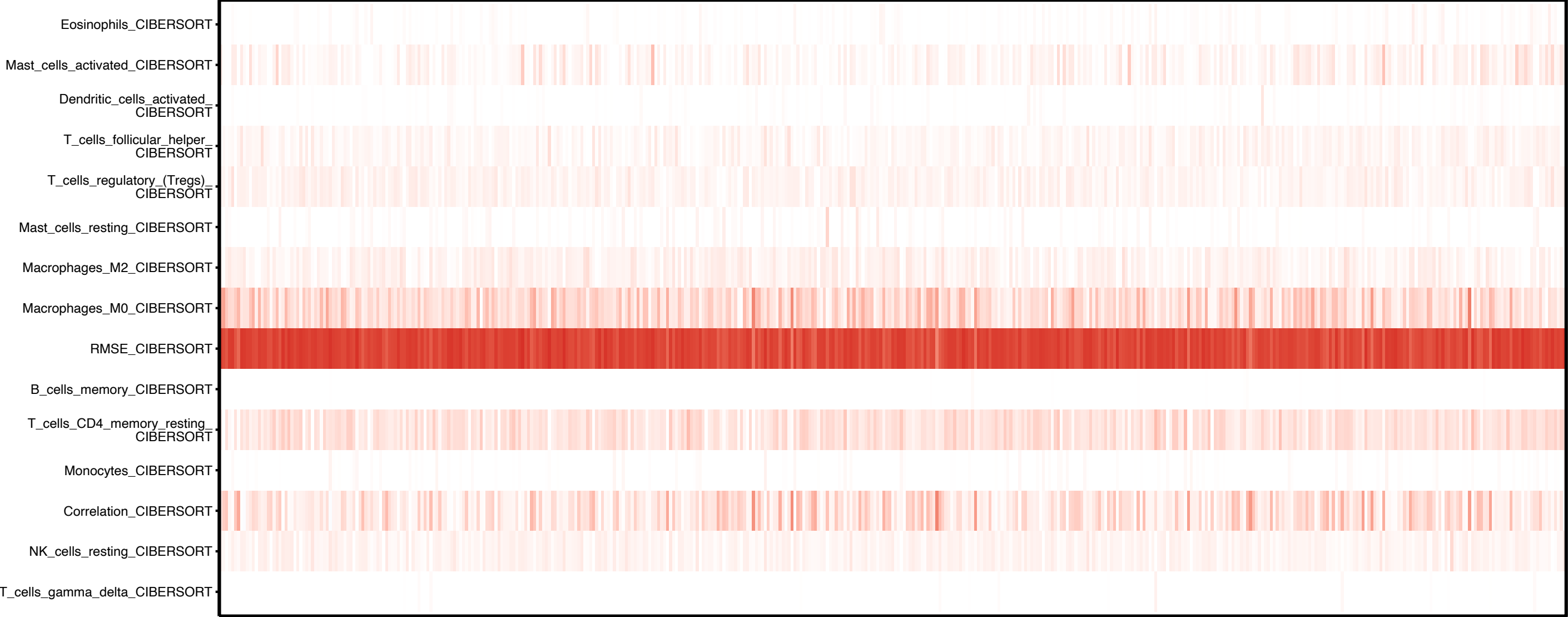
TCGA_COAD_01A_ATF3_svr top feature heatmap
