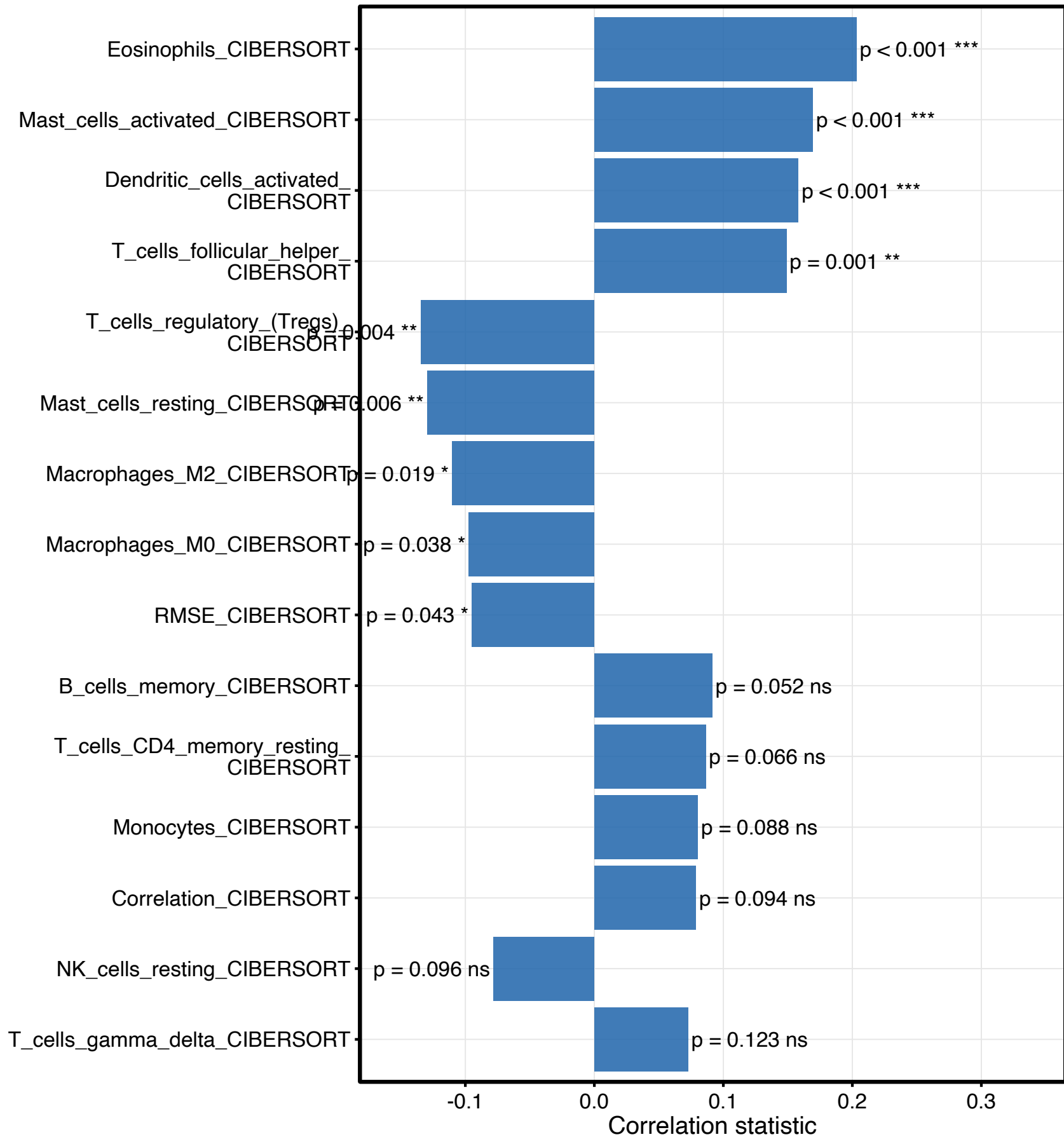
TCGA_COAD_01A_ATF3_svr correlation with target gene
