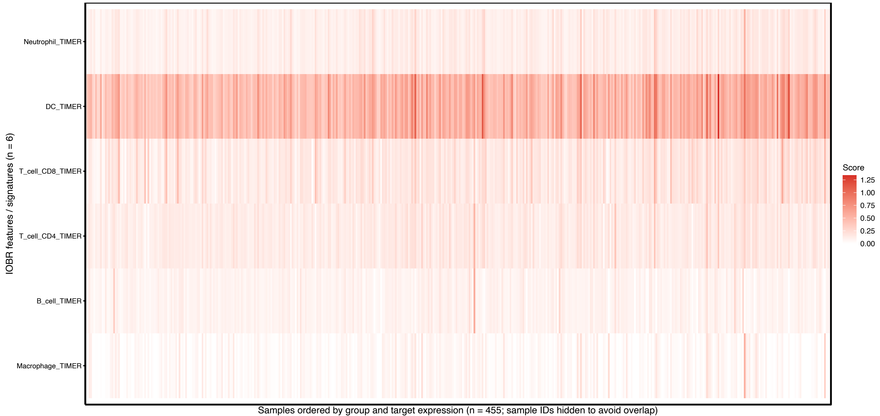
TCGA_COAD_01A_ATF3_timer all IOBR features heatmap
