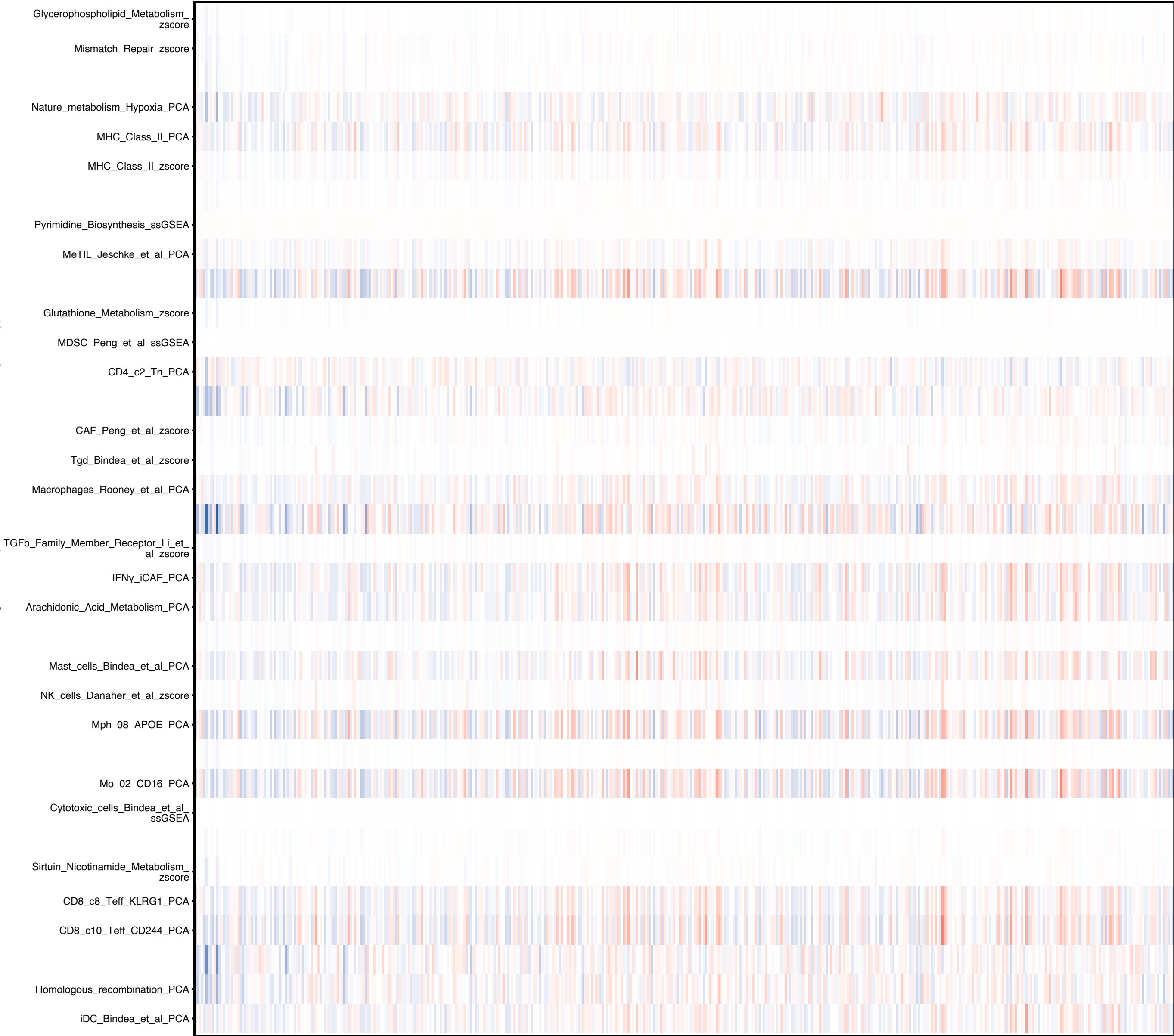
TCGA_COAD_01A_ATF3_integration all IOBR features heatmap part 014/026
