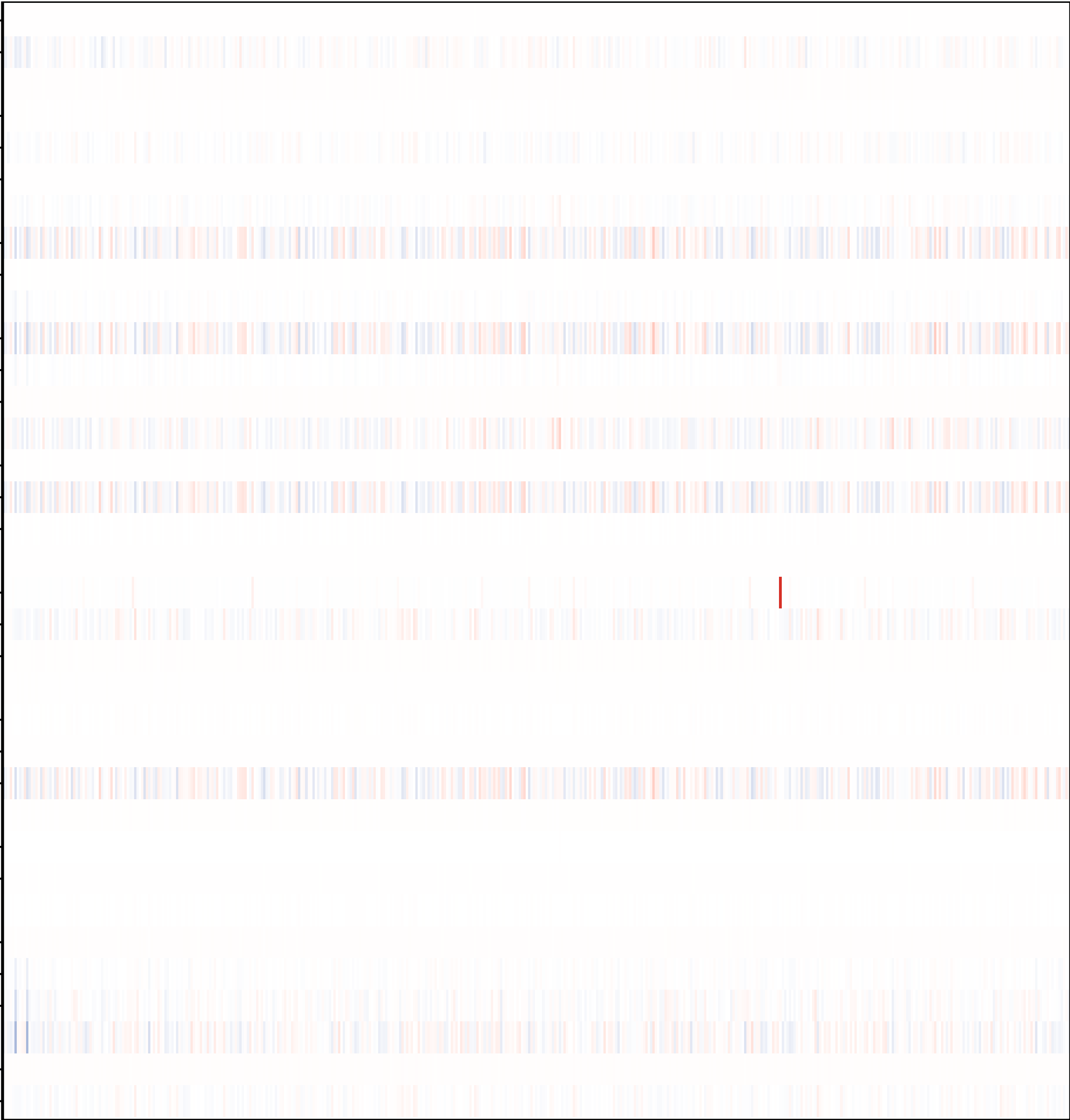
TCGA_COAD_01A_ATF3_integration all IOBR features heatmap part 022/026
