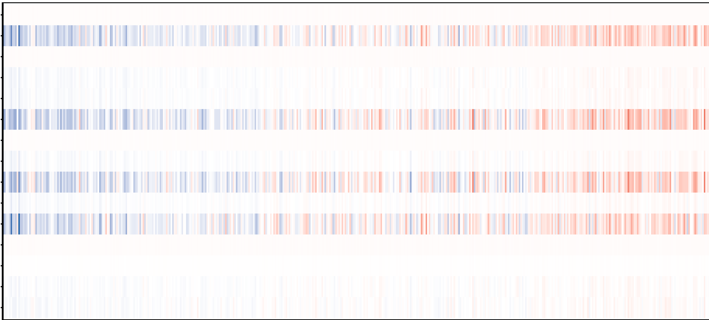
TCGA_COAD_01A_ATF3_integration top feature heatmap
