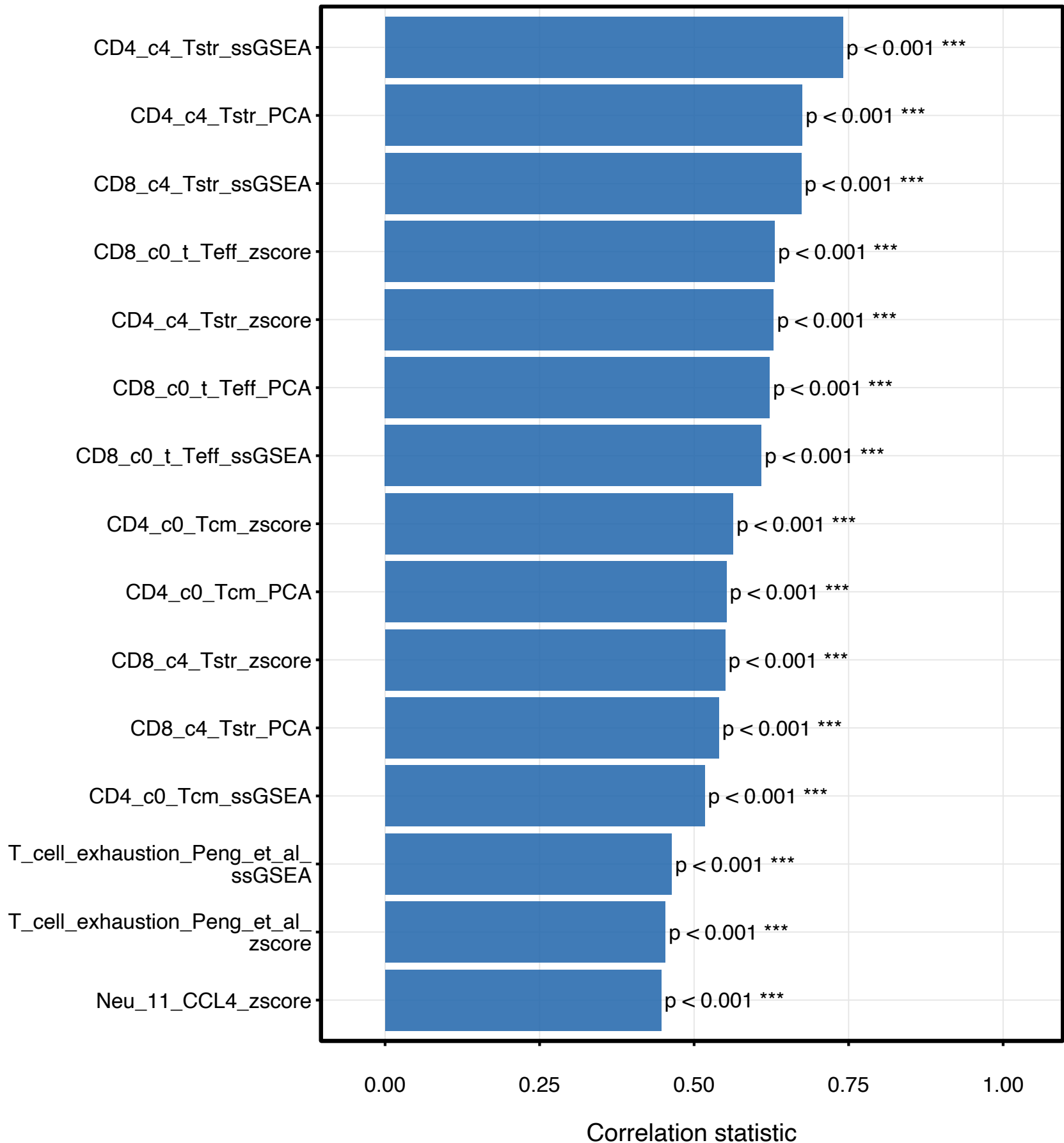
TCGA_COAD_01A_ATF3_integration correlation with target gene
