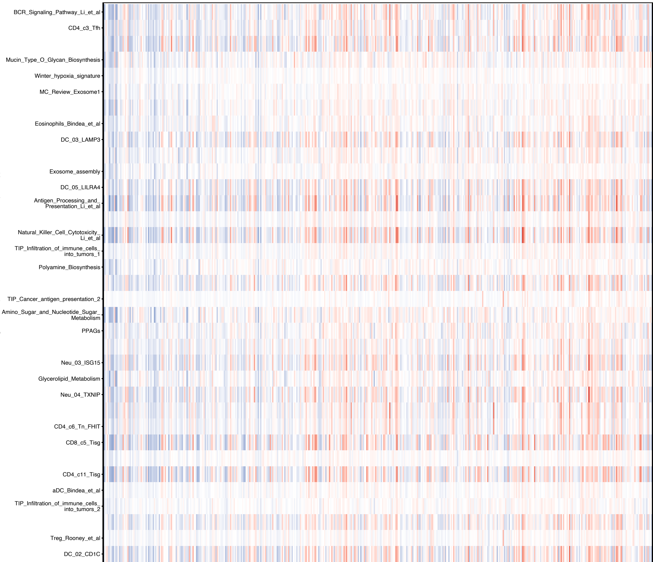
TCGA_COAD_01A_ATF3_pca all IOBR features heatmap part 002/009
