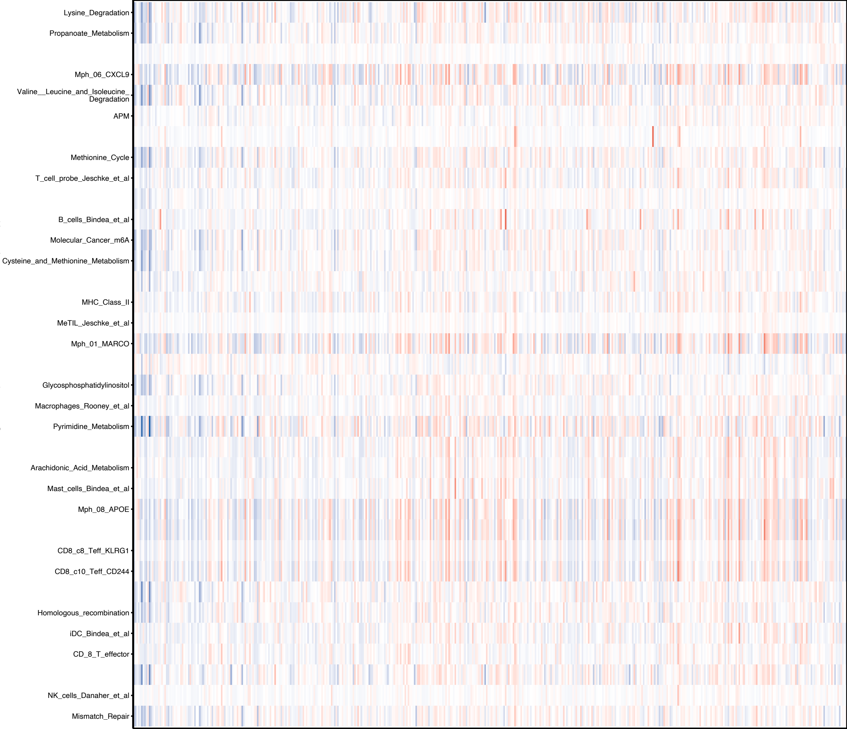
TCGA_COAD_01A_ATF3_pca all IOBR features heatmap part 006/009
