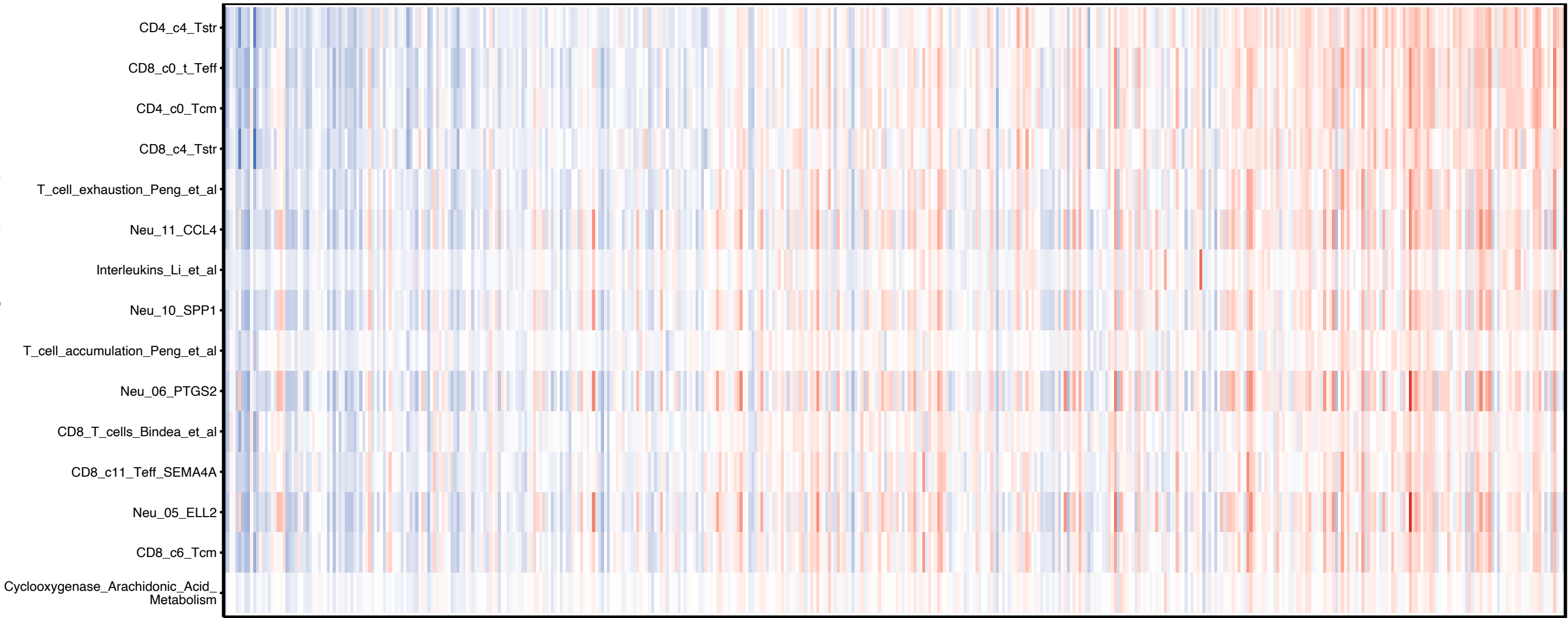
TCGA_COAD_01A_ATF3_pca top feature heatmap
