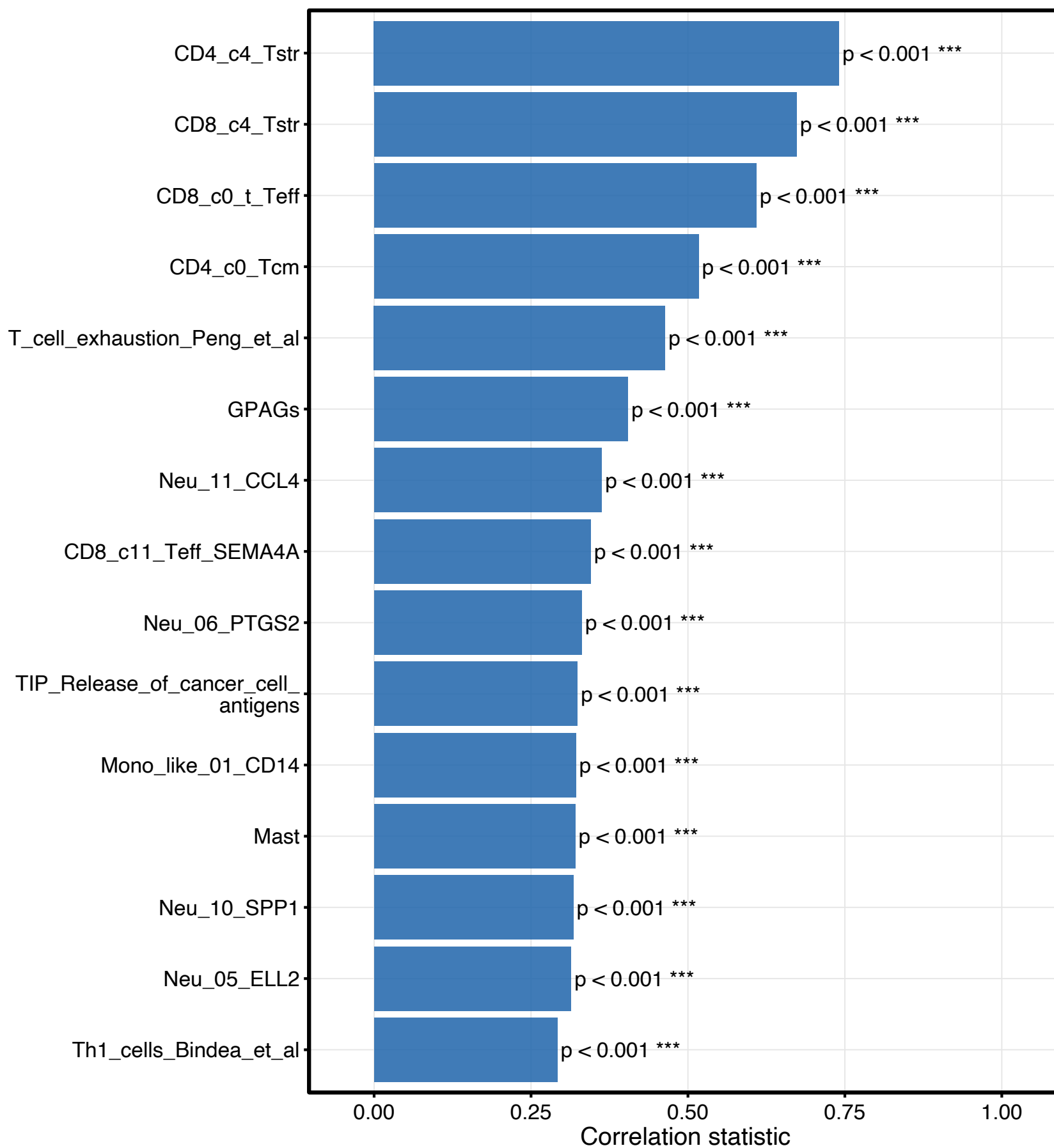
TCGA_COAD_01A_ATF3_ssgsea correlation with target gene
