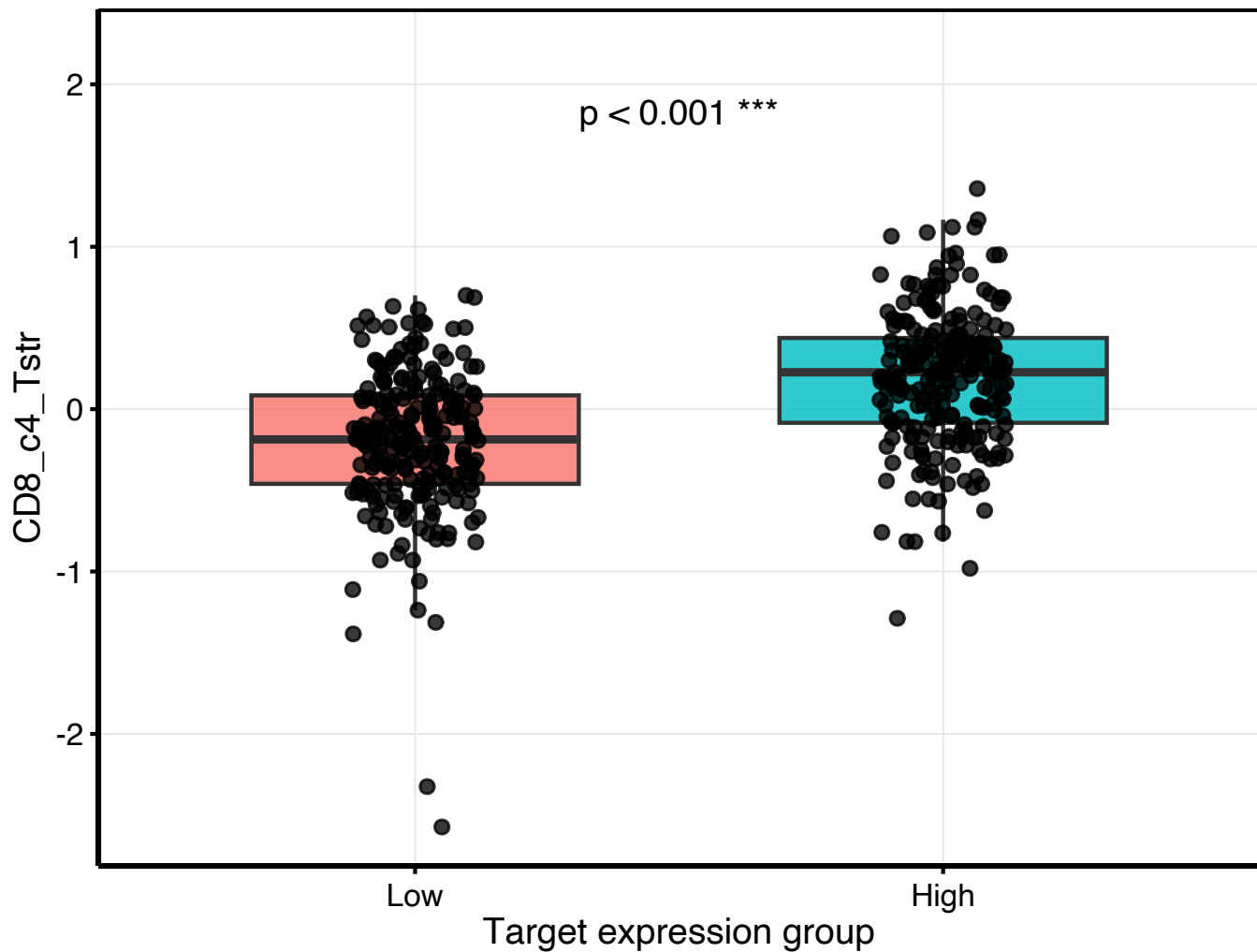
TCGA_COAD_01A_ATF3_zscore CD8_c4_Tstr by Target expression group
