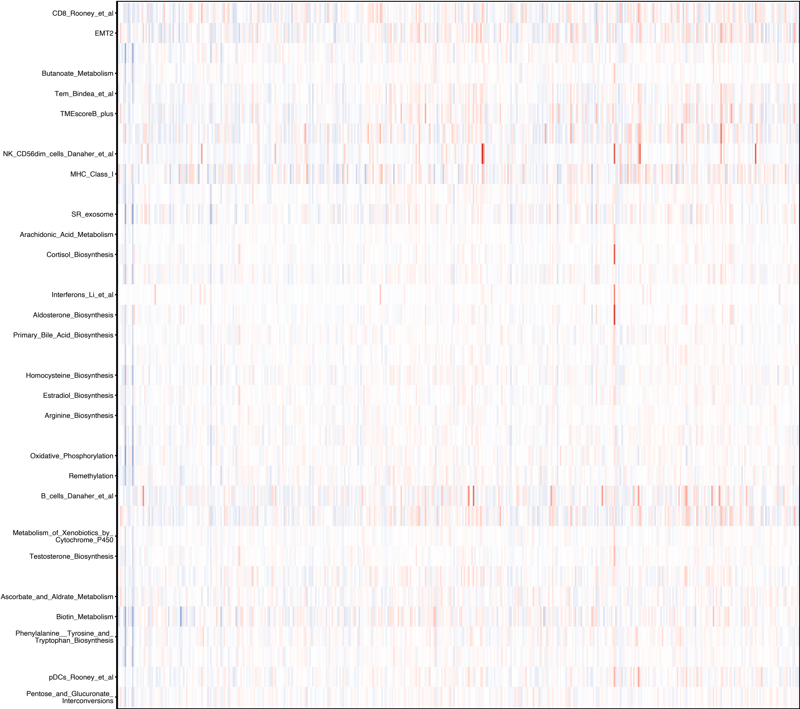
TCGA_COAD_01A_ATF3_zscore all IOBR features heatmap part 008/009
