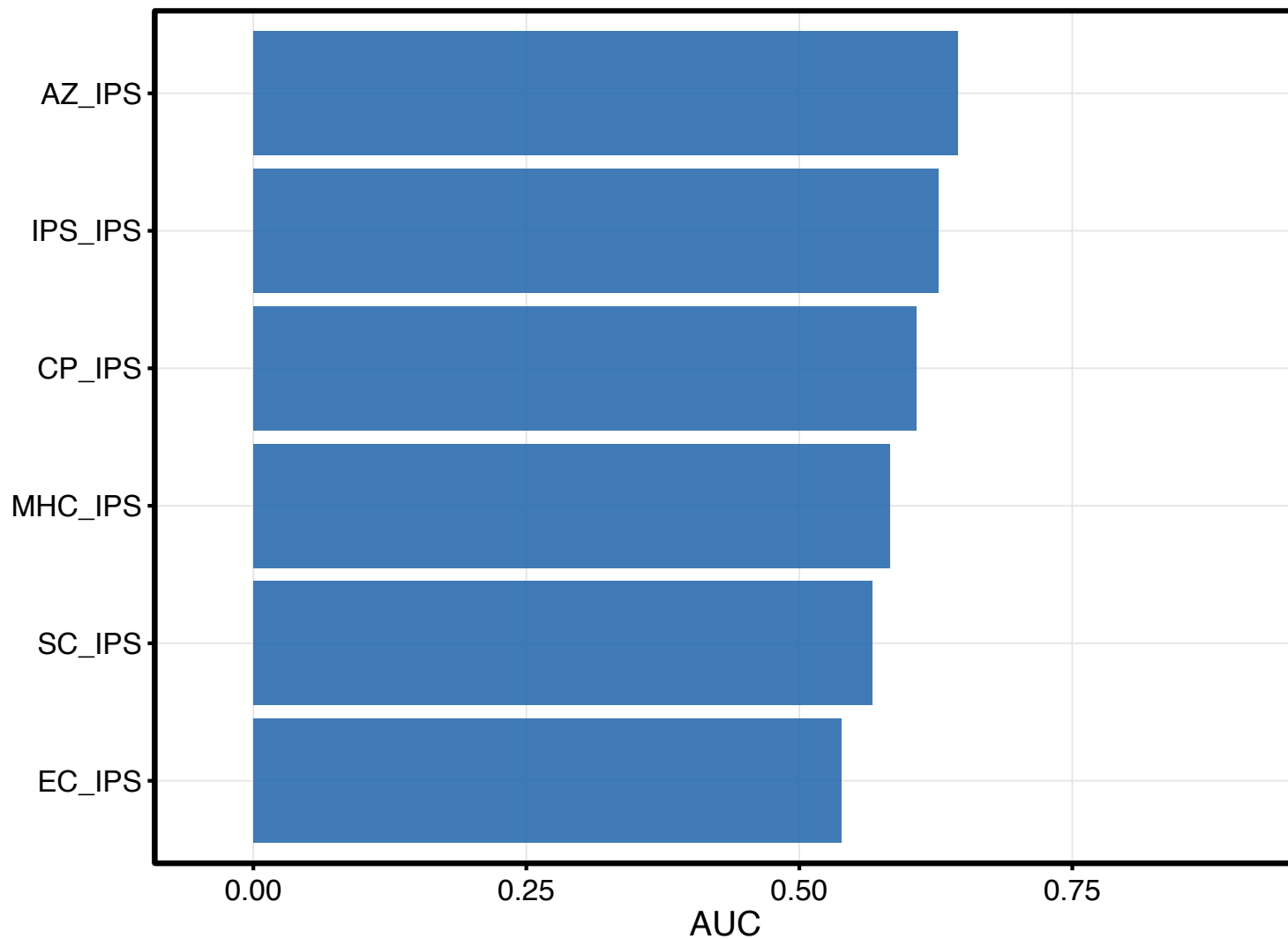
GTEx_COLON_ATF3_ips_scores Target_Group ROC
