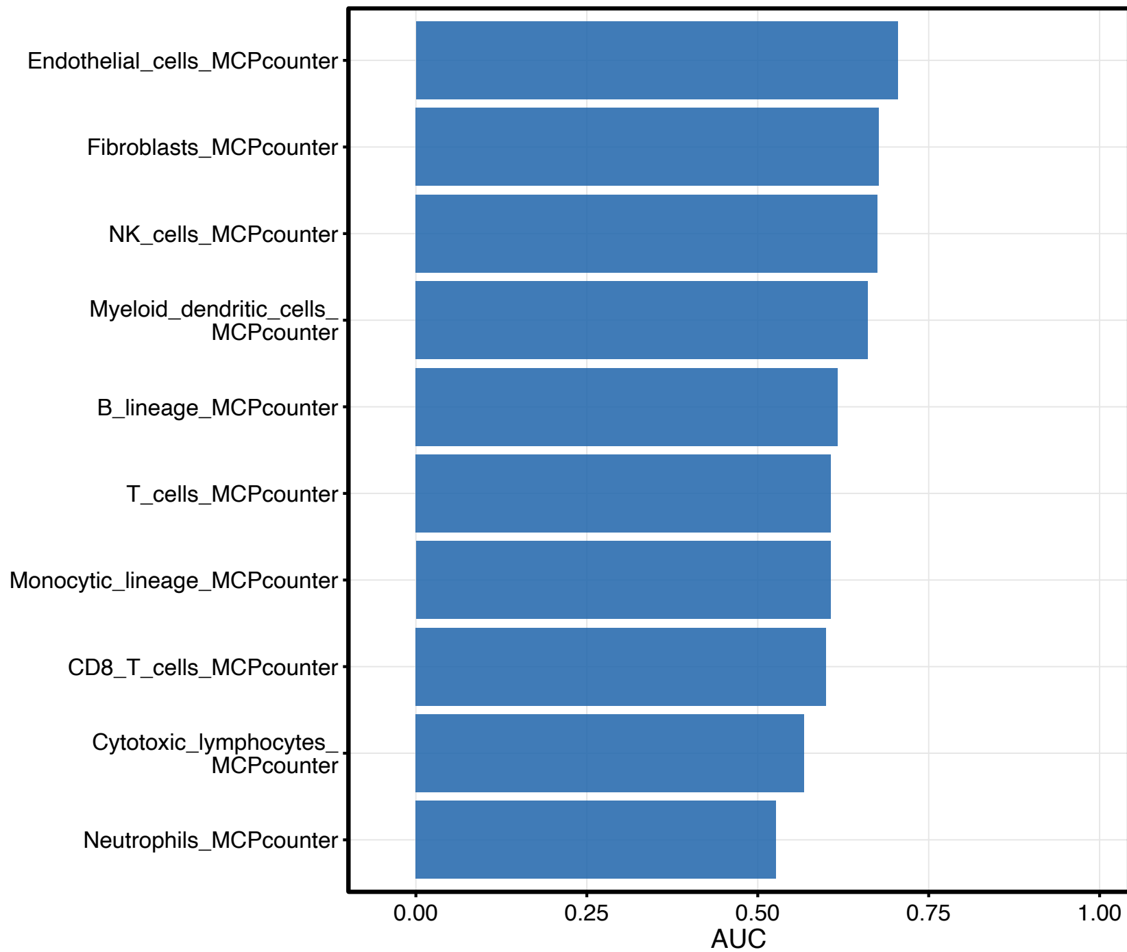
GTEx_COLON_ATF3_mcpcounter_scores Target_Group ROC
