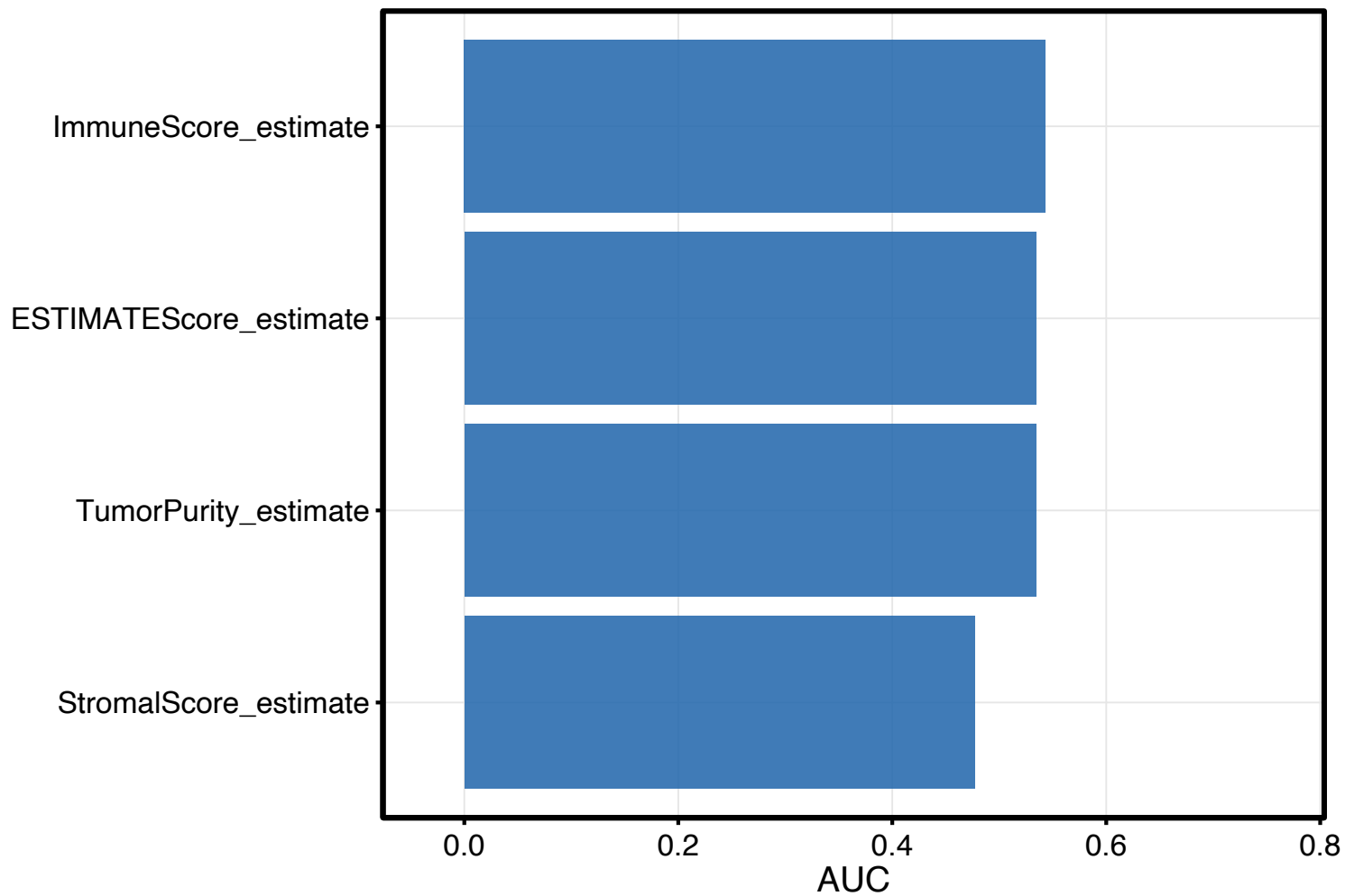
TCGA_COAD_01A_ATF3_estimate_scores Target_Group ROC
