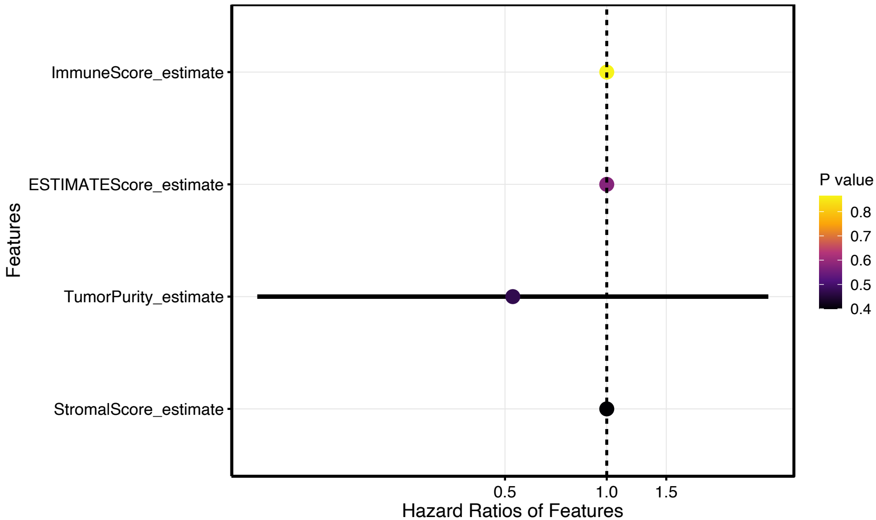
TCGA_COAD_01A_ATF3_estimate_scores survival forest
