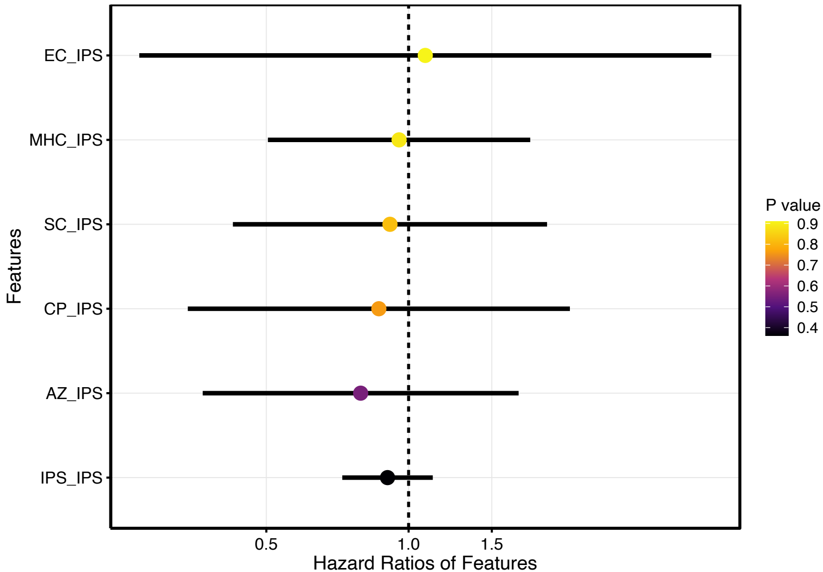
TCGA_COAD_01A_ATF3_ips_scores survival forest
