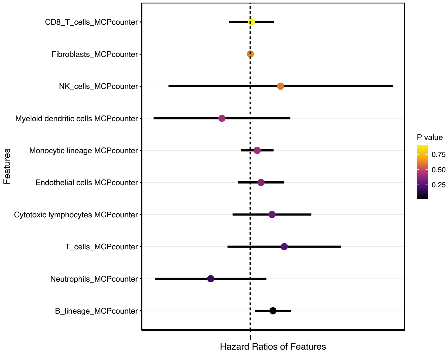
TCGA_COAD_01A_ATF3_mcpcounter_scores survival forest
