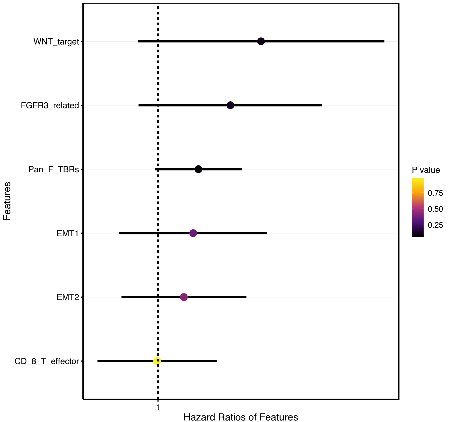
TCGA_COAD_01A_ATF3_pca_scores survival forest
