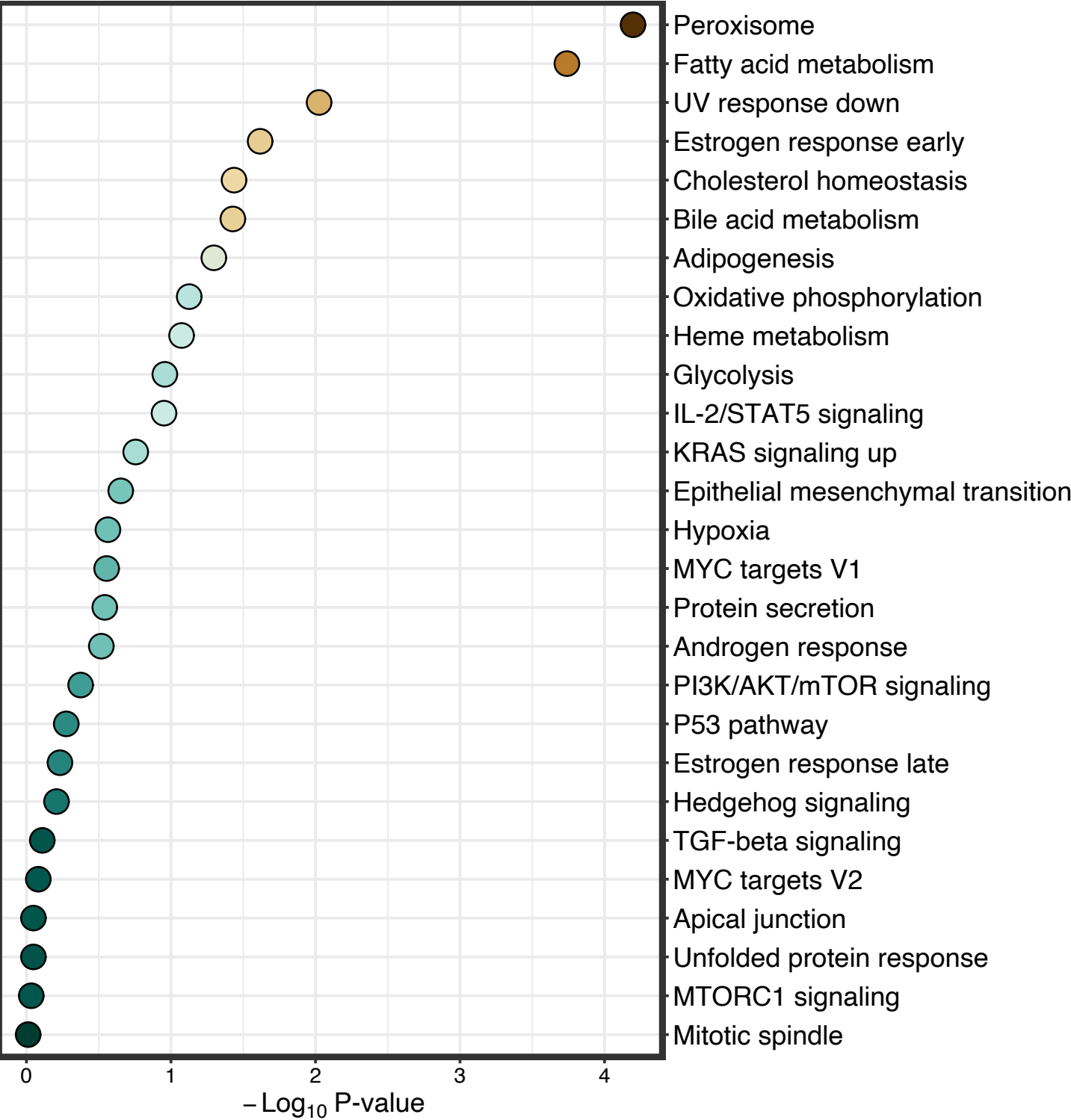
Positive Terms (Mutation vs WildType)
