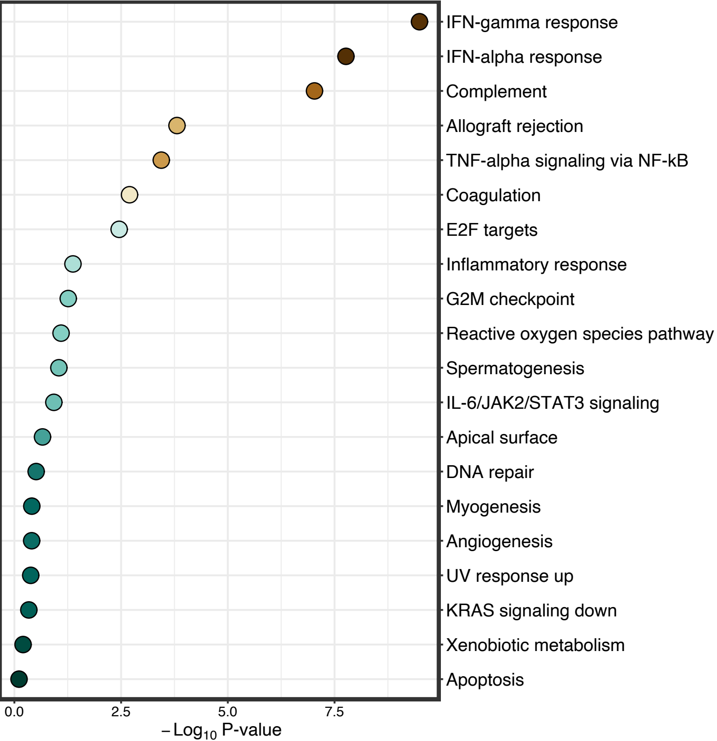
Negative Terms (Mutation vs WildType)
