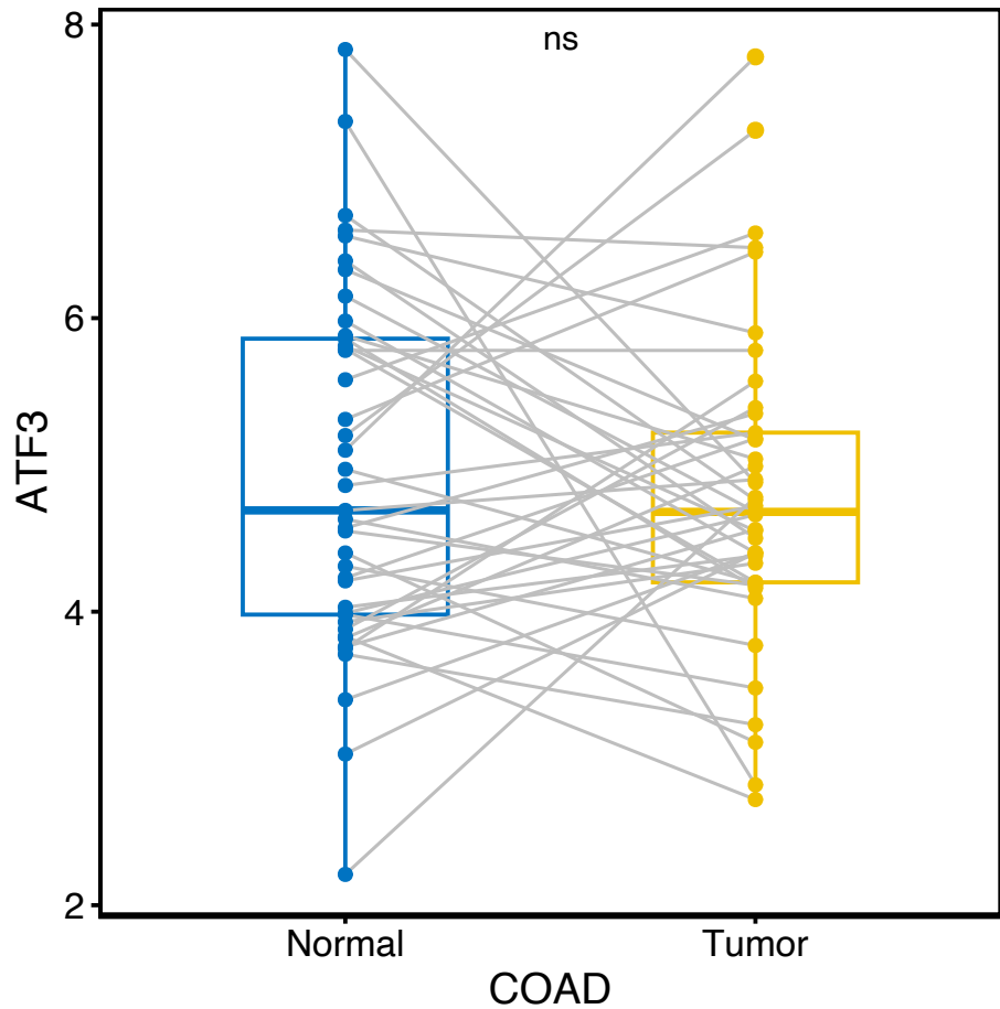
paired boxplot | ATF3 | COAD
