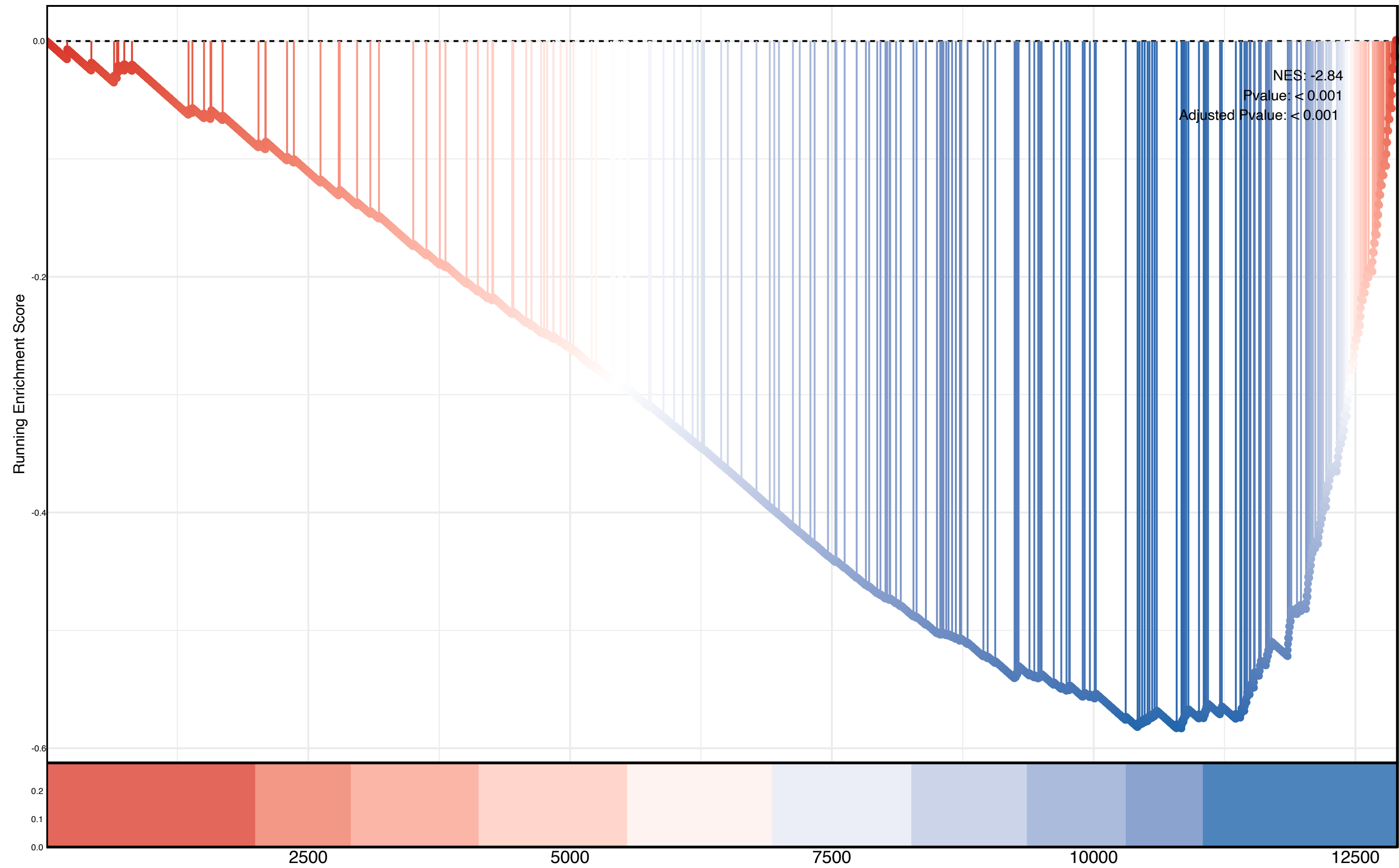
Condensed Chromosome
