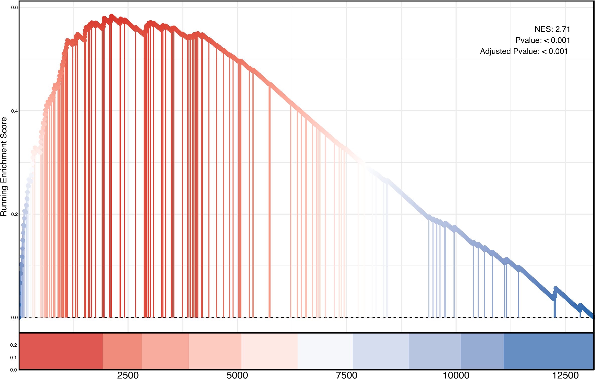
Anti Trem1 Vs Vehicle Treated Monocytes Up
