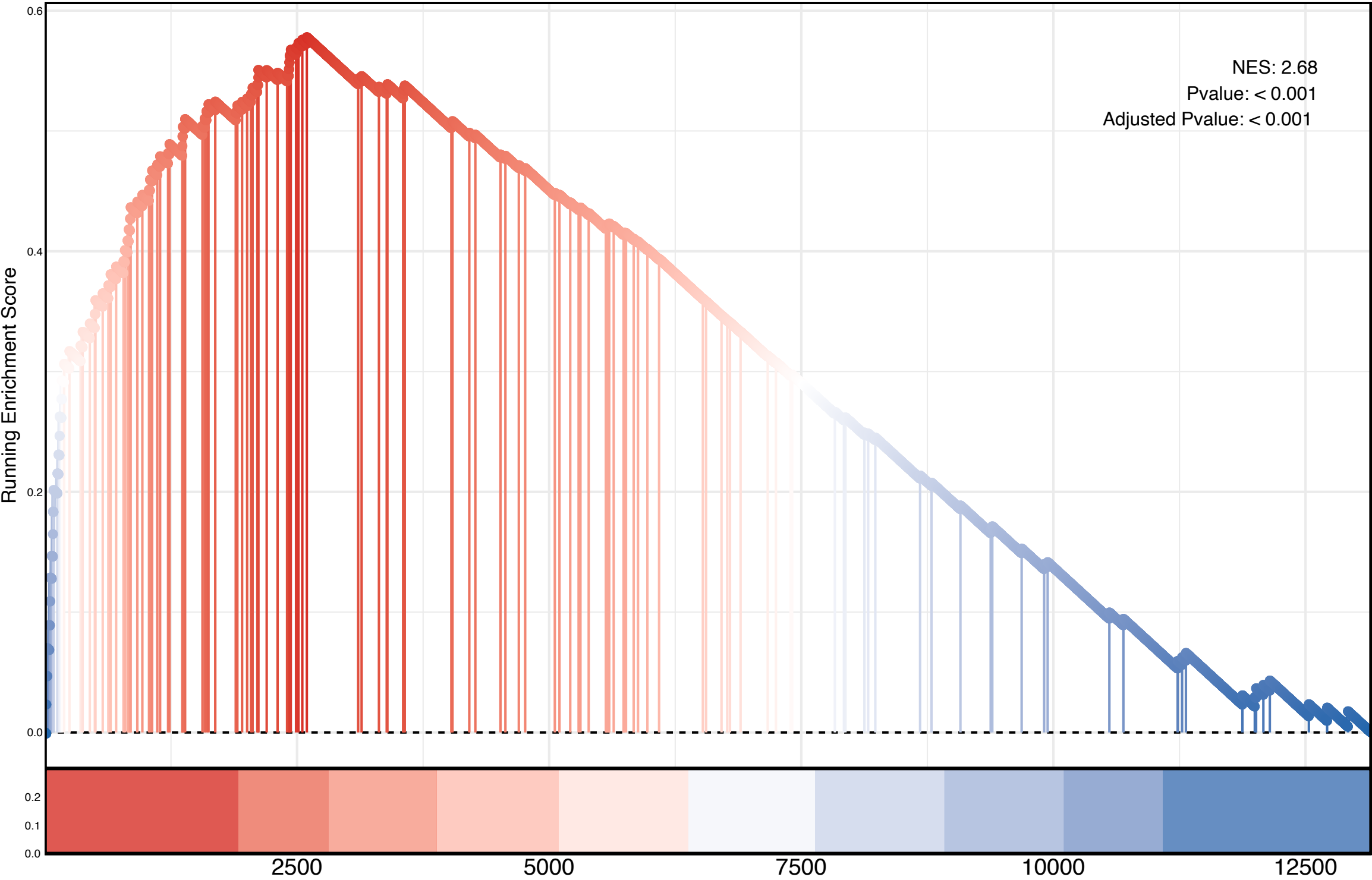
Unstim Vs 2h Lps Dc Dn
