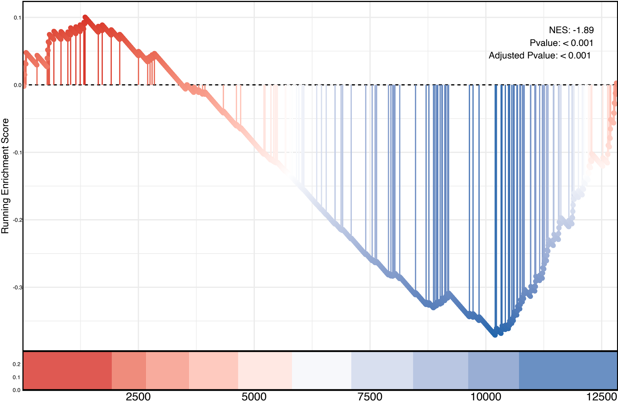
Proton Transmembrane Transporter Activity
