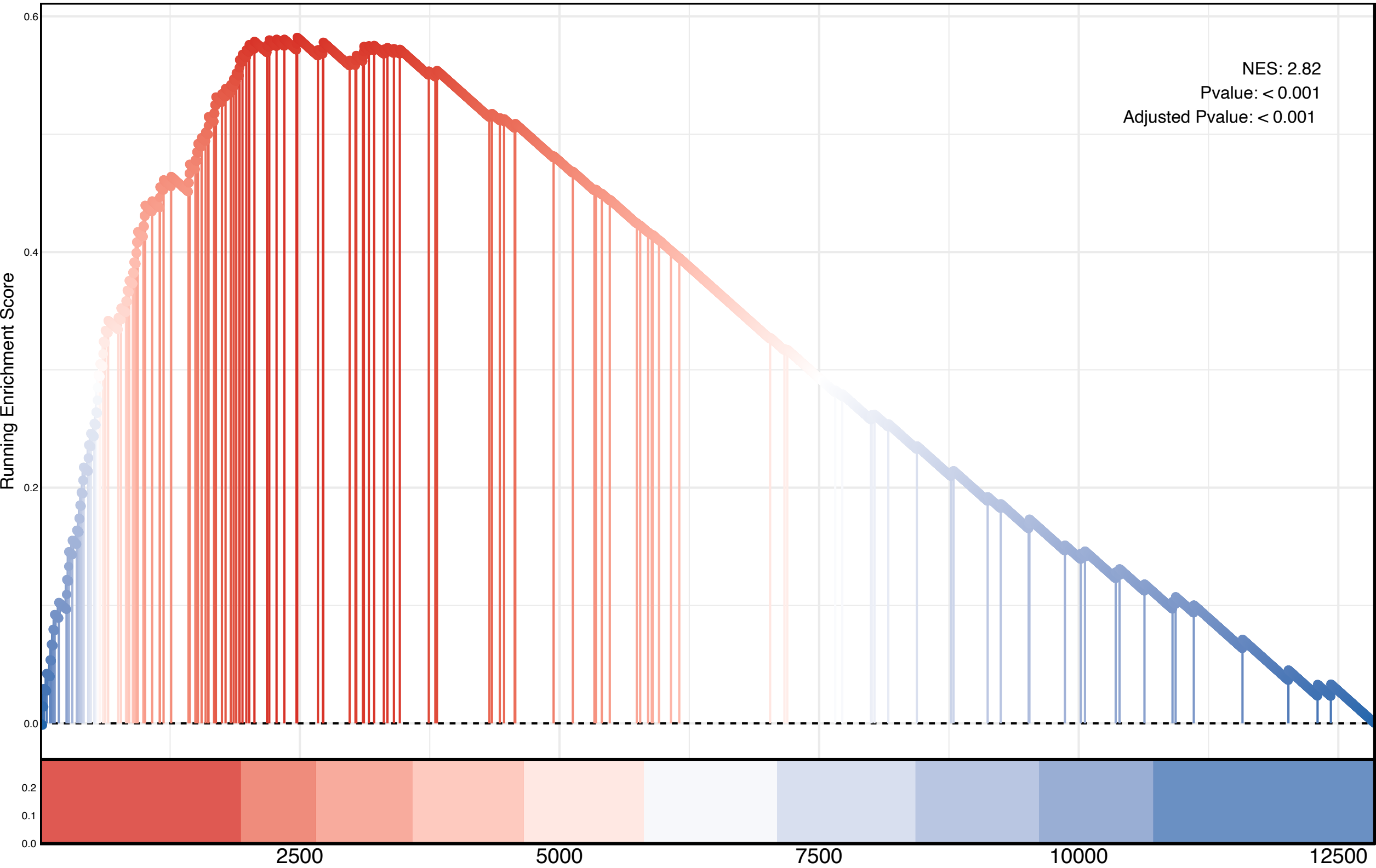
Anti Trem1 And Lps Vs Ctrl Treated Monocytes Up
