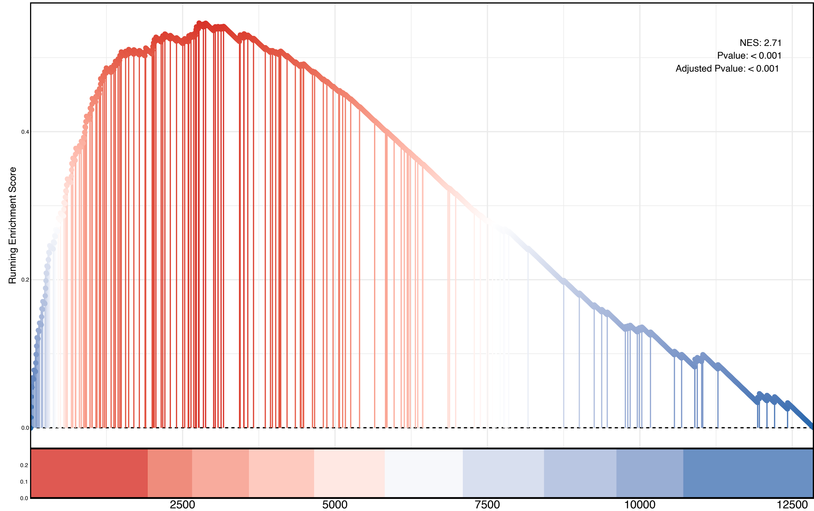
Ctrl Vs 24h F Tularensis Lvs Neutrophil Dn
