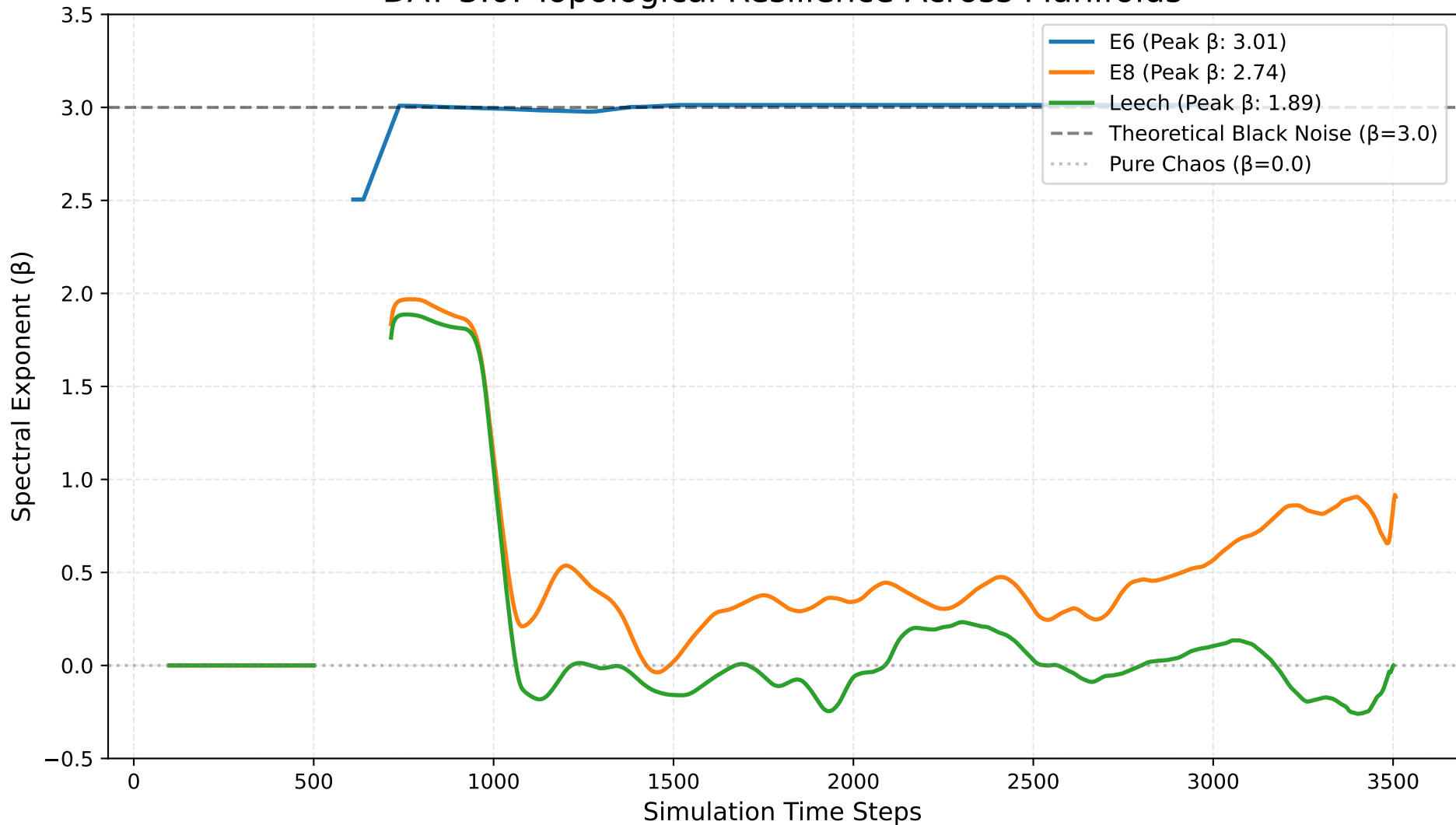
DAT 3.0: Topological Resilience Across Manifolds
