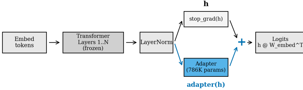
Figure 3: Post-transformer adapter placement. Hidden states from the frozen model are gradient-detached ( stop_grad ). The adapter receives gradients through the manual logit projection h @ W_{\text{embed}}^T . No transformer weights are modified.
