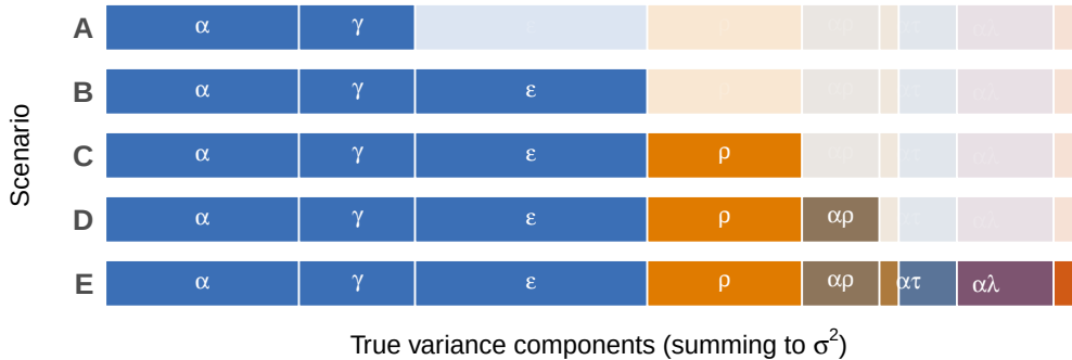
(b) Variance budget: which components each SE accounts for
