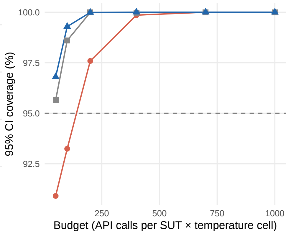
(b) CI coverage of oracle
