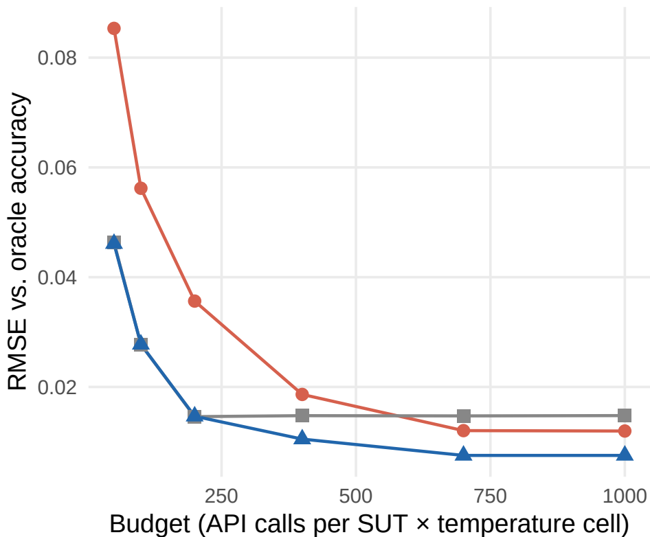
(a) Estimation accuracy
