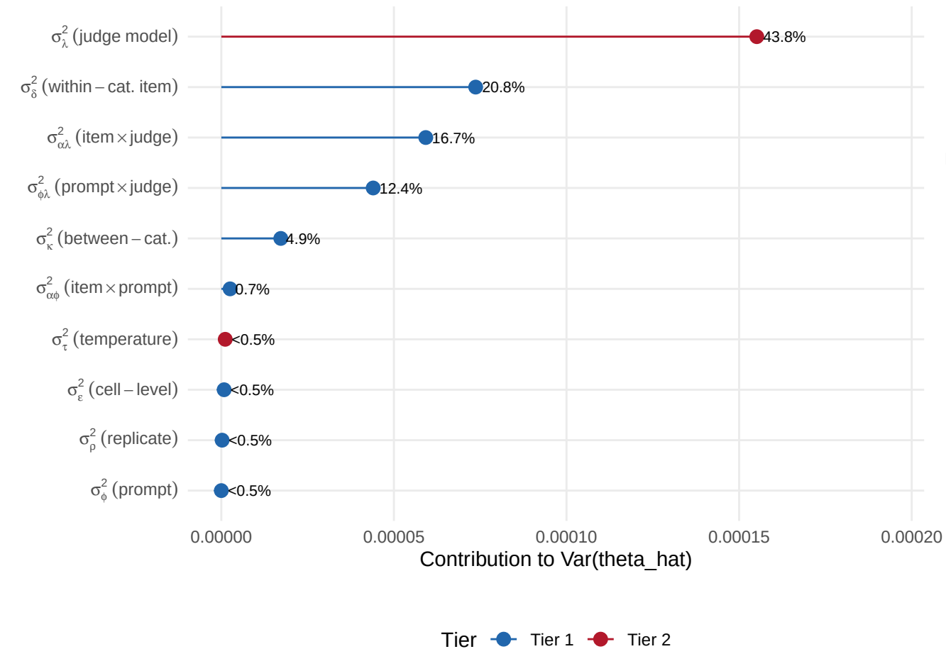
(a) Var(theta_hat) Decomposition (Safety: SAFE/UNSAFE)
