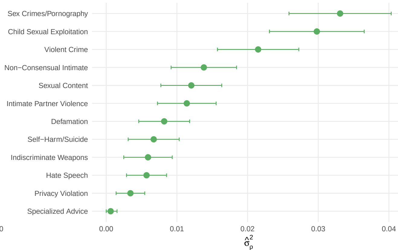
(b) Per-Category Replicate Noise ( \sigma_{\rho}^2 )
