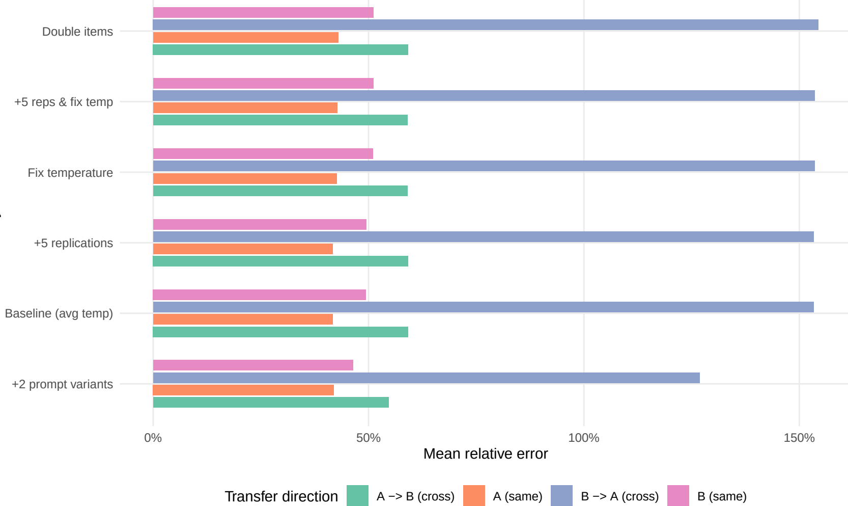
D-Study Transfer Prediction Error Relative |\text{predicted} - \text{actual}| / \text{actual} (N_SIM=1000)
