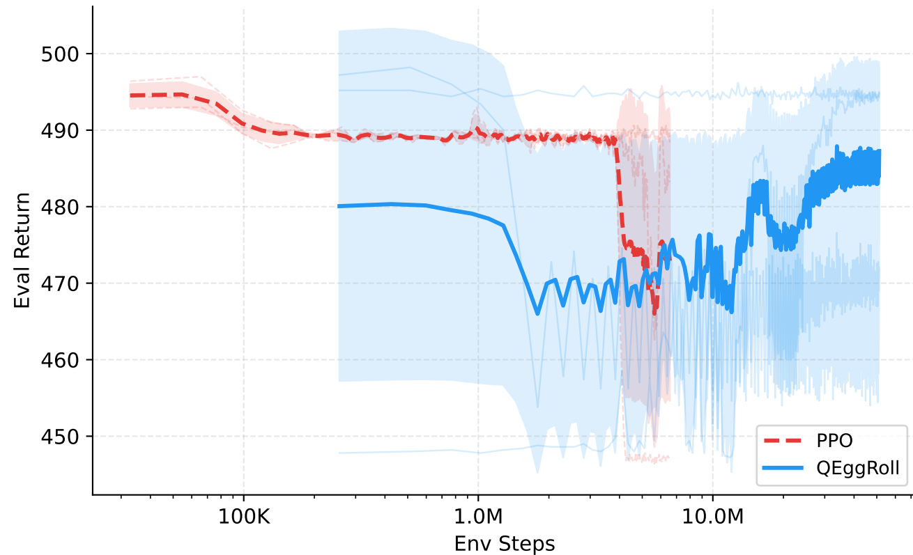
Sample Efficiency (log x-axis)
