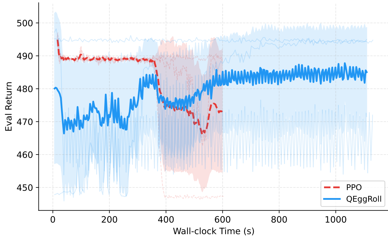
Computational Efficiency
