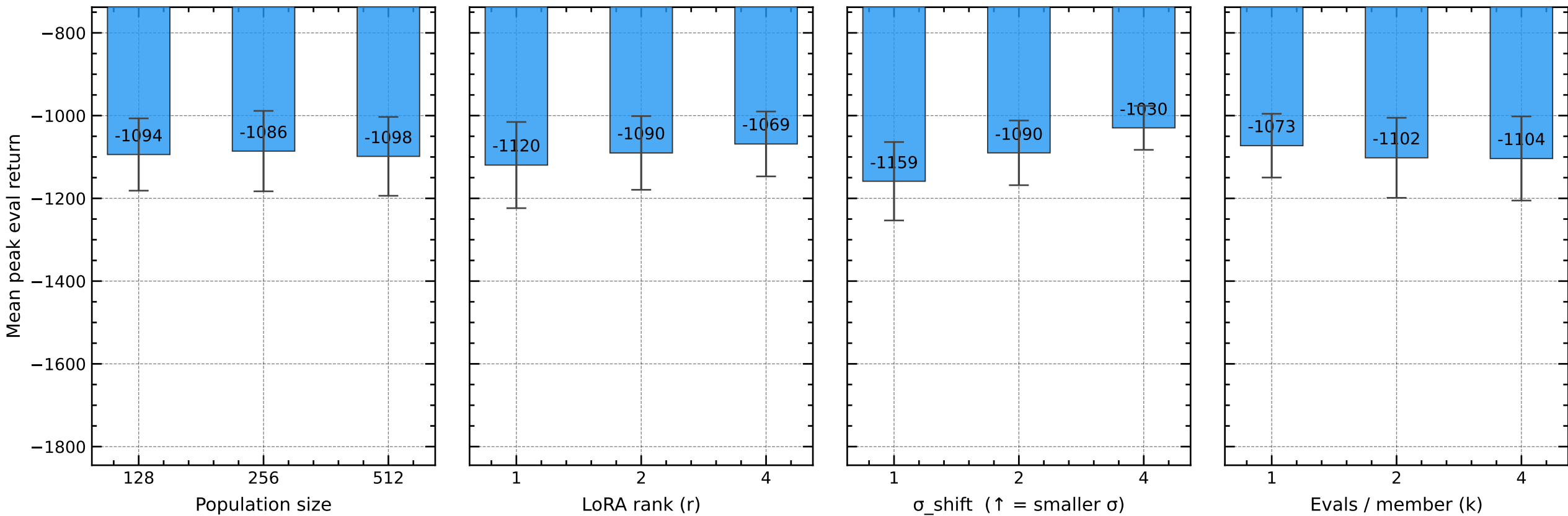
Marginal hyperparameter effect — Pendulum-v1 (mean peak eval return across 27 configurations per bar; error bars = std)
