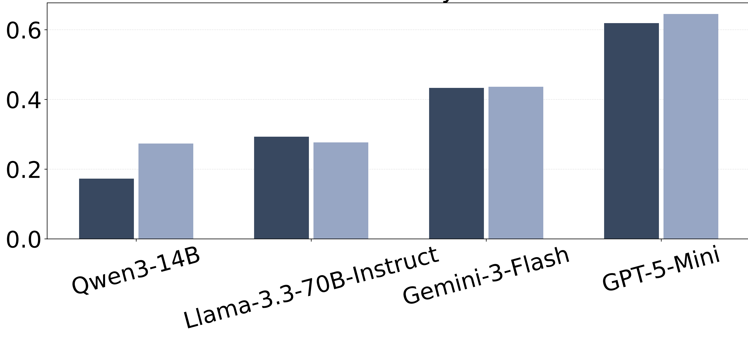
Accuracy
