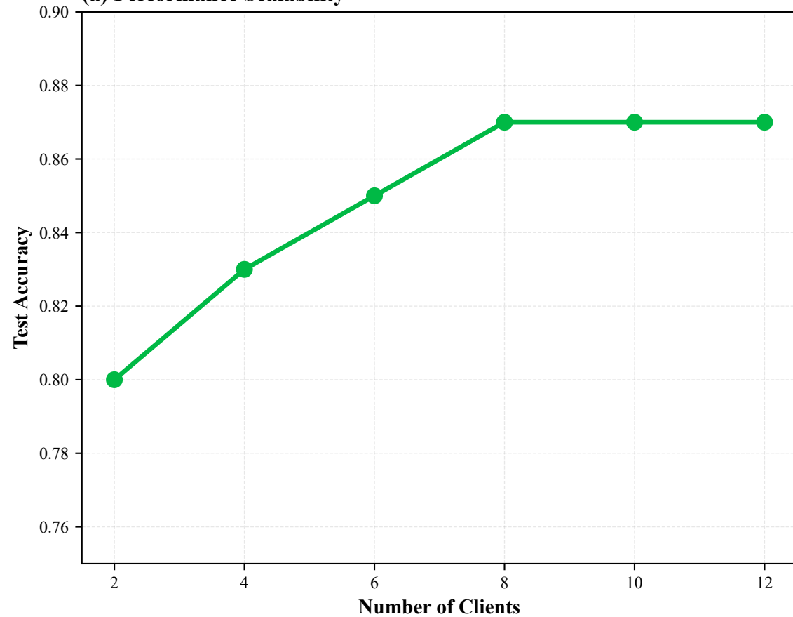
(a) Performance Scalability
