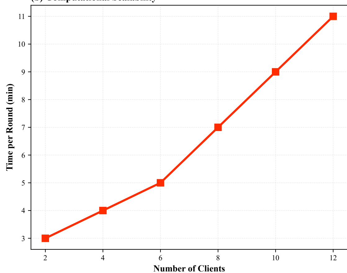
(b) Computational Scalability
