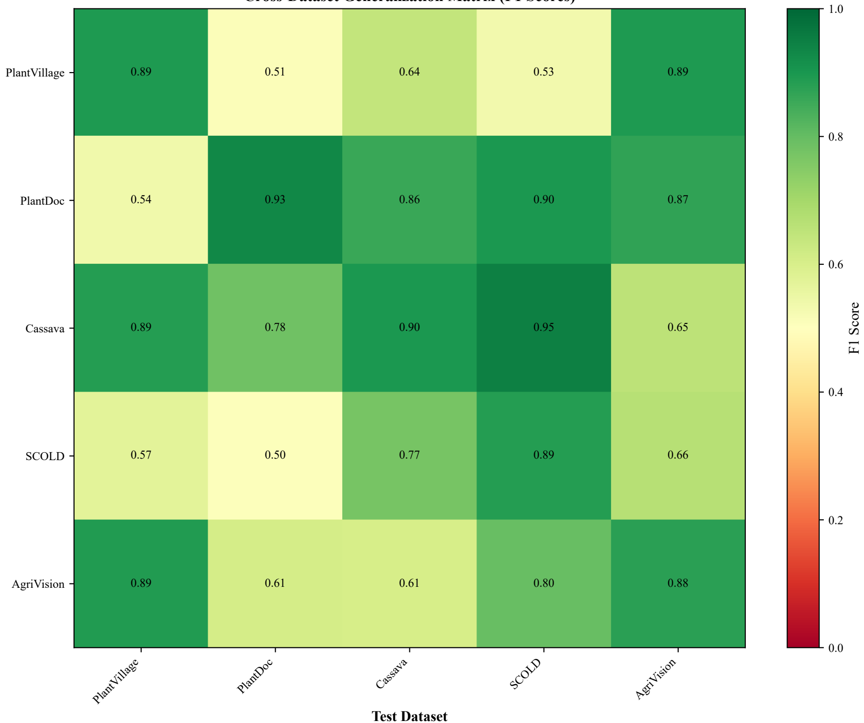
Cross-Dataset Generalization Matrix (F1 Scores)
