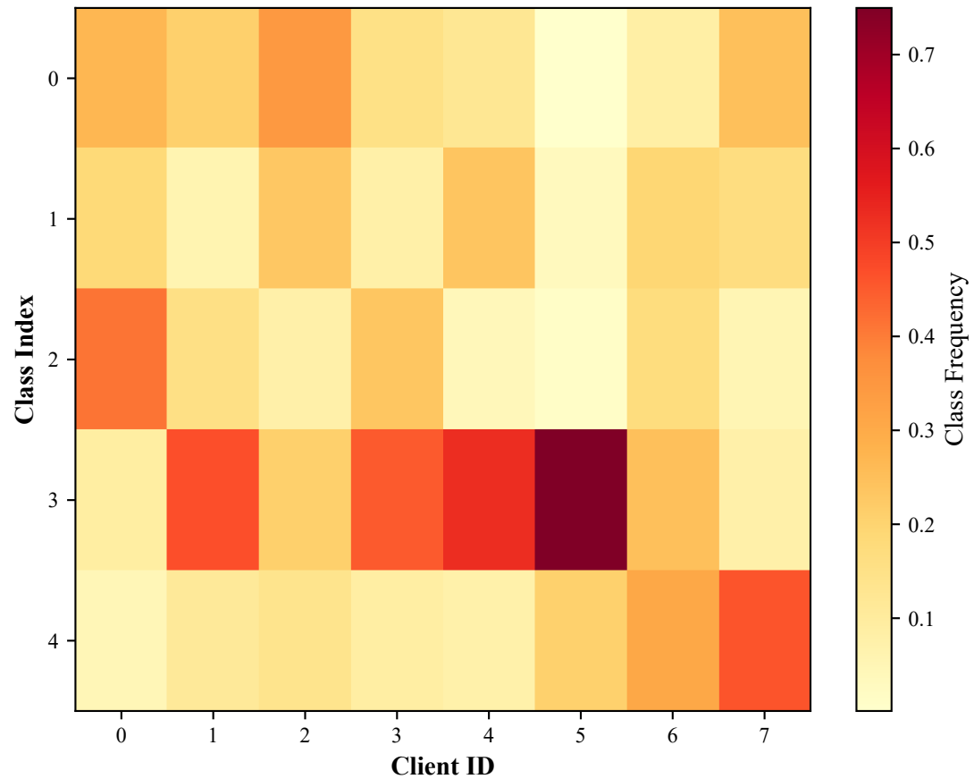
(b) Class Distribution Heatmap
