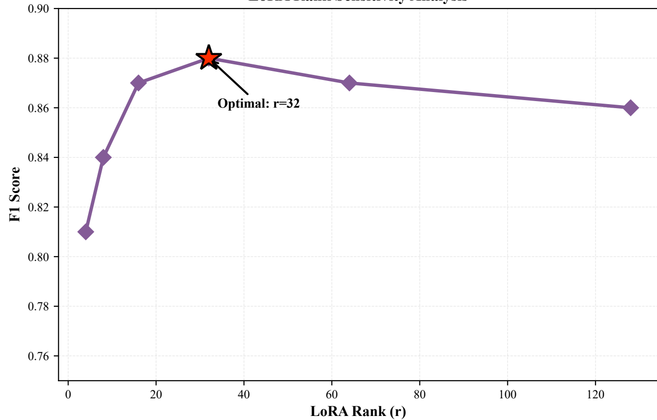
LoRA Rank Sensitivity Analysis
