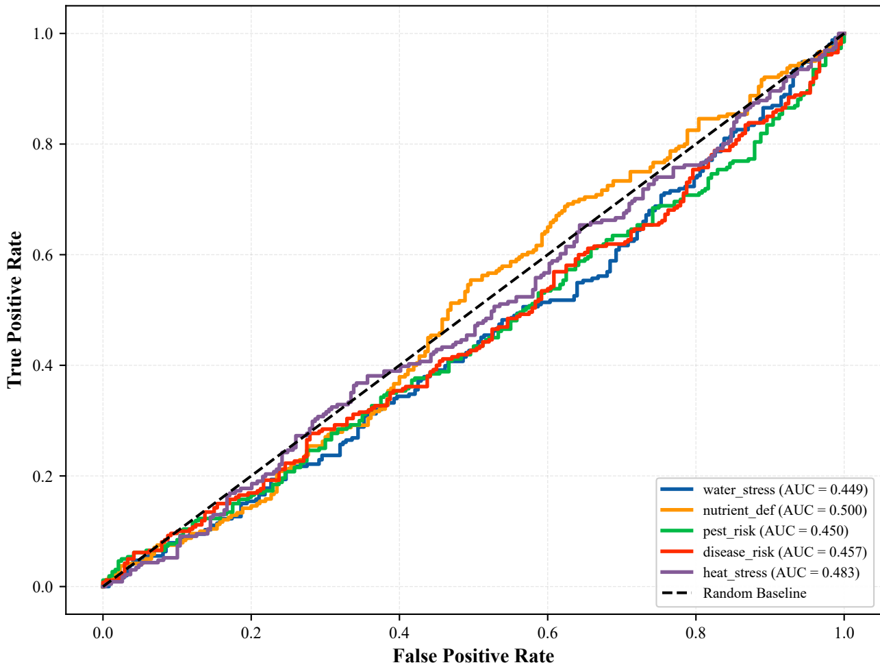
ROC Curves: Per-Class Performance
