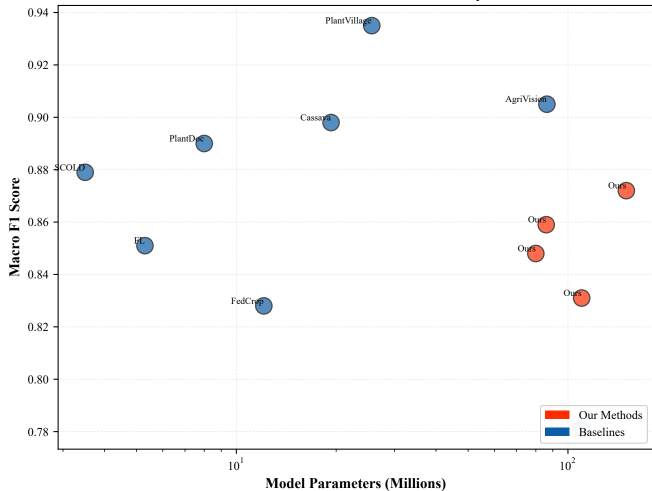
Performance vs Parameter Efficiency
