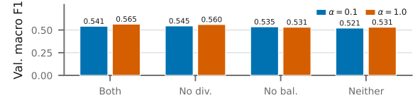
Fig. 10: Anti-collapse arms at both skews, from zero because the finding is that none of them collapses. Values are printed: the arms span 0.044, all of it the balanced sampler, and the diversity term does nothing.
