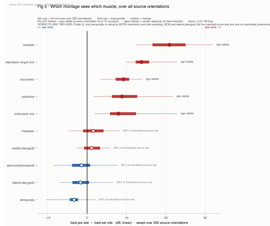
Figure 5: Which montage sees which muscle. For each articulator, the difference between the best jaw site and the best retroauricular site, in dB. Negative bars are muscles the ear sees more strongly. Jaw sites within 10 mm of the truncation face are excluded. The shaded band is the measured electrode-meshing floor (0.27 dB, with the lighter band extending to its 95 % CI upper bound of 0.65 dB). The axis is linear in dB rather than a rank, because the asymmetry between the arms is itself a result: the jaw's advantages reach +20.90 dB while the ear's reach only −3.31 dB. Both numbers are emitted from the figure's own source file by src/04m_caption_numbers.py, which fails the build if a caption and its figure disagree.
