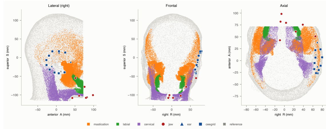
Fig. 1. MIDA head model with the ten segmented articulator compartments highlighted, and all 22 electrode positions shown in lateral, frontal and axial views. The face is removed anterior of the eyes at all heights, in accordance with MIDA licence clause 2.3.3.
