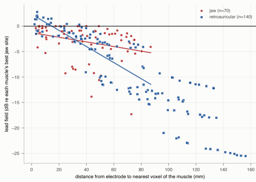
Fig. 5. Attenuation against source-electrode distance. One point per (electrode, muscle) pair: straight-line distance from the electrode to the nearest voxel of that muscle compartment against the lead field in dB relative to that muscle's best jaw site, isotropic condition, truncated mesh. The two montages do not lie on the same attenuation curve. Fitted over the 3 to 87 mm range where both montages have electrodes, the retroauricular sites fall off at -0.158 dB/mm against the jaw's -0.045 dB/mm, a factor of 3.5 [results/04s_fig3_slopes.csv]. A retroauricular electrode therefore loses signal with distance more than three times as fast as a jaw electrode does, which is the geometric mechanism behind the labial-group deficit reported in §4.3. Lines are least-squares fits over the overlapping range only, so the comparison is made where both montages have data, not extrapolated across the ear's longer reach.
