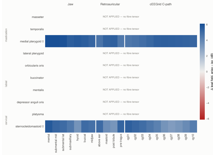
Fig. 4. Anisotropy robustness check. Change in lead field between the isotropic and anisotropic conditions, 20 \cdot \log_{10}(\text{aniso}/\text{iso}) , per cell. The anisotropic condition is solved on the isotropic run's own mesh, so the two differ in conductivity alone and carry no electrode-realisation noise. A fibre tensor is applied to 2 of 10 muscles, sternocleidomastoid and medial pterygoid. Rows without a tensor are labelled not applied, not zero: they were never varied, so no null result was measured for them.
