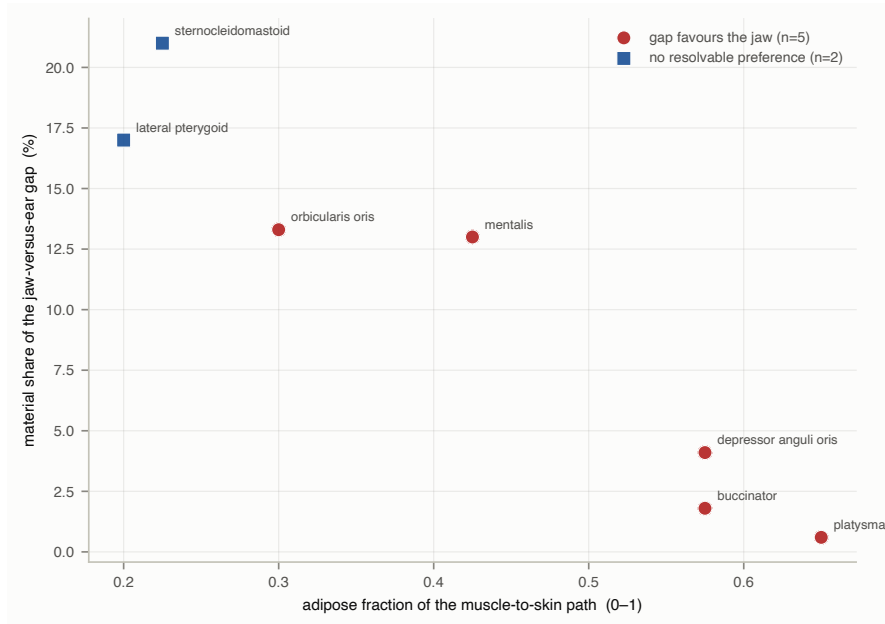
Fig. 6. Material share falls as the adipose path grows. For each of the seven muscles with a layer profile, the adipose fraction of the muscle-to-skin path against the material share of that muscle's jaw-versus-ear gap. The relationship is negative (Spearman \rho = -0.955 , p = 0.001 , n = 7 ): more fat on the path means a smaller material share, not a larger one, because a muscle embedded uniformly in fat has both the jaw and the ear route shifted together and the change cancels in the ratio. Leave-one-out leaves \rho between -0.928 and -0.986 with p below 0.01 in every case, so no single muscle carries it. Points are marked by whether the muscle's gap resolves to the jaw or reaches no resolvable preference. No trend line is drawn: these are seven independent muscles, not a series, and Spearman is a rank statistic that claims no functional form.
