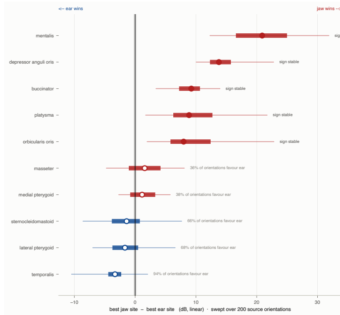
Fig. 3. Which montage sees which muscle. For each articulator, the difference between the best jaw site and the best retroauricular site, in dB. Negative bars are muscles the ear sees more strongly. Jaw sites within 10 mm of the truncation face are excluded. The shaded band is the measured electrode-meshing floor (0.27 dB, with the lighter band extending to its 95 % CI upper bound of 0.65 dB). The axis is linear in dB and not a rank, because the asymmetry between the arms is itself a result: the jaw's advantages reach +20.90 dB while the ear's reach only -3.31 dB. Both numbers are emitted from the figure's own source file by src/04m_caption_numbers.py , which fails the build if a caption and its figure disagree.
