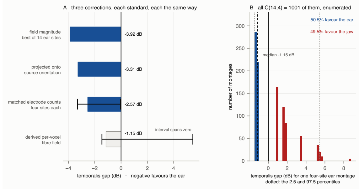
Fig. 10. How the retroauricular advantage dissolved. Left : the temporalis gap at four stages, each read from the file that reproduces it: field magnitude against the best of fourteen ear sites, then projected onto source orientation, then at matched electrode counts, then under the fibre field derived from the label volume. Rules are matched-count intervals where one exists. Each correction is individually standard, none was applied in response to the result, and only the last interval spans zero. Right : what that last interval is made of. The ear pool holds 14 sites and a montage takes 4, giving exactly C(14,4) = 1001 possible retroauricular montages, every one of which is enumerated here, so the histogram is the population, not a sample of it. Dotted lines are the 2.5 and 97.5 percentiles quoted as the interval; 28.6 per cent of montages attain the lower bound exactly, which is why that bound coincides with the floor.
