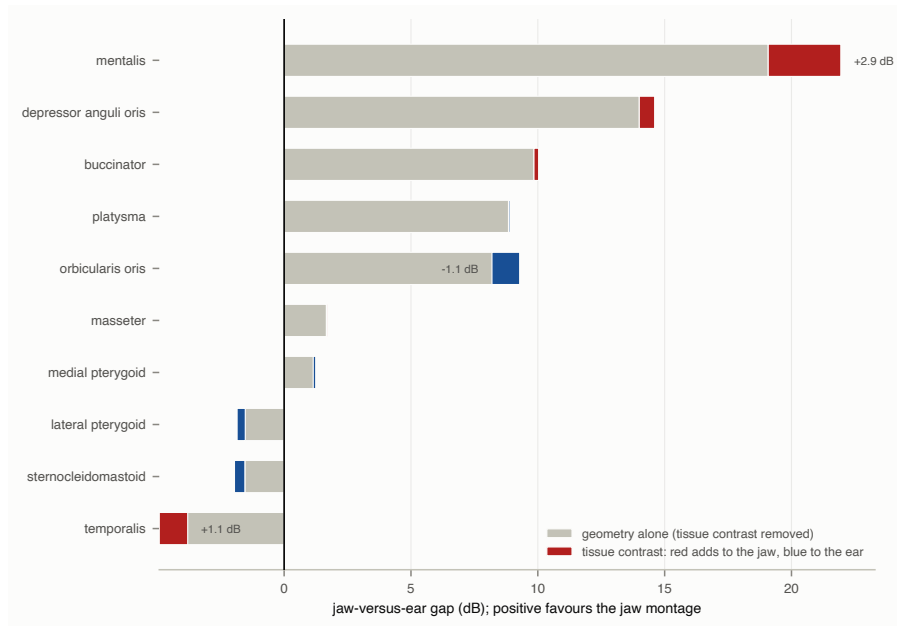
Fig. 7. Geometry sets the gap, tissue only trims it. Each muscle’s jaw-versus-ear gap split into the part that survives when the adipose-muscle conductivity contrast is removed, with geometry held exactly fixed, and the part that does not. Positive is a jaw advantage. The geometric term reaches 19.1 dB; the material term never exceeds 2.9 dB and changes sign, moving five muscles toward the jaw and five toward the ear. A single material share for the set would average that sign change away, which is why the text reports shares muscle by muscle.
