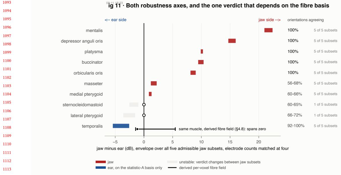
Fig. 11. Both robustness axes, and the one verdict that depends on the basis. Table 4 drawn: one bar per muscle spanning the envelope over all five admissible jaw subsets, with electrode counts matched at four, coloured by verdict, against the orientation-agreement range on the right. Five muscles sit entirely on the jaw side on both axes. Two are unstable, changing verdict between jaw subsets, and their bars cross zero. Temporalis sits entirely on the ear side on the statistic-A basis used for Table 4, which takes the median over a uniform 200-direction orientation sweep. The black rule beneath it is the same comparison under the per-voxel fibre field derived from the label volume, which spans zero. It is the only row that carries a second rule, because it is the only muscle whose verdict depends on which basis is used, and §4.8 gives the argument for preferring the derived field.
