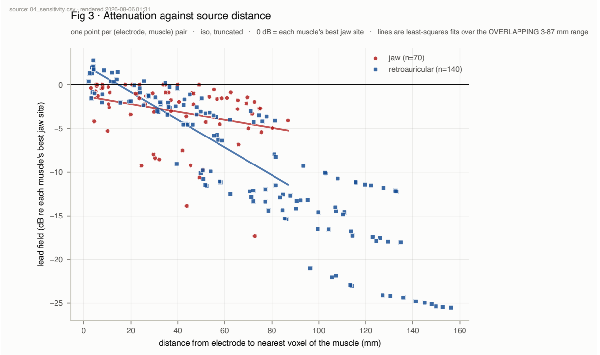
Figure 3: Attenuation against source-electrode distance. One point per (electrode, muscle) pair: straight-line distance from the electrode to the nearest voxel of that muscle compartment against the lead field in dB relative to that muscle's best jaw site, isotropic condition, truncated mesh. The two montages do not lie on the same attenuation curve. Fitted over the 3 to 87 mm range where both montages have electrodes, the retroauricular sites fall off at -0.158 dB/mm against the jaw's -0.045 dB/mm, a factor of 3.5 [results/04s_fig3_slopes.csv]. A retroauricular electrode therefore loses signal with distance more than three times as fast as a jaw electrode does, which is the geometric mechanism behind the labial-group deficit reported in §4.3. Lines are least-squares fits over the overlapping range only, so the comparison is made where both montages have data rather than extrapolated across the ear's longer reach.
