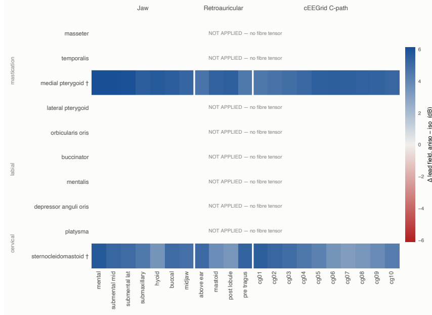
Fig. 4. Anisotropy robustness check. Change in lead field between the isotropic and anisotropic conditions, 20\text{-log}_{10}(\text{aniso}/\text{iso}) , per cell. The anisotropic condition is solved on the isotropic run’s own mesh, so the two differ in conductivity alone and carry no electrode-realisation noise. A fibre tensor is applied to 2 of 10 muscles, sternocleidomastoid and medial pterygoid. Rows without a tensor are labelled not applied, not zero: they were never varied, so no null result was measured for them.
