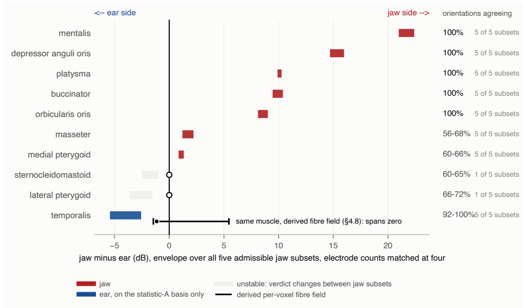
Fig. 11. Both robustness axes, and the one verdict that depends on the basis. Table 4 drawn: one bar per muscle spanning the envelope over all five admissible jaw subsets, with electrode counts matched at four, coloured by verdict, against the orientation-agreement range on the right. Five muscles sit entirely on the jaw side on both axes. Two are unstable, changing verdict between jaw subsets, and their bars cross zero. Temporalis sits entirely on the ear side on the statistic-A basis used for Table 4, which takes the median over a uniform 200-direction orientation sweep. The black rule beneath it is the same comparison under the per-voxel fibre field derived from the label volume, which spans zero. It is the only row that carries a second rule, because it is the only muscle whose verdict depends on which basis is used, and §4.8 gives the argument for preferring the derived field.
