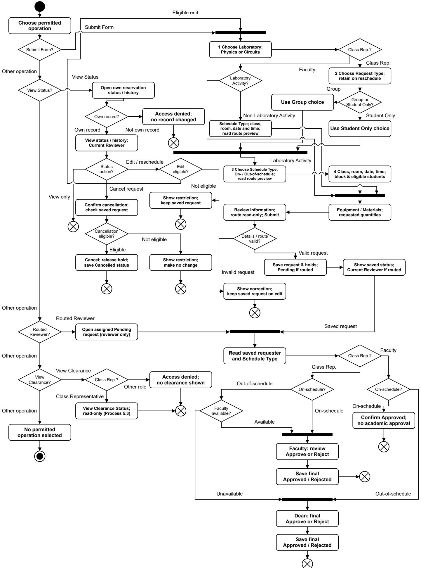
Figure 12: Activity Diagram - Manage Reservations, Availability & Approvals
