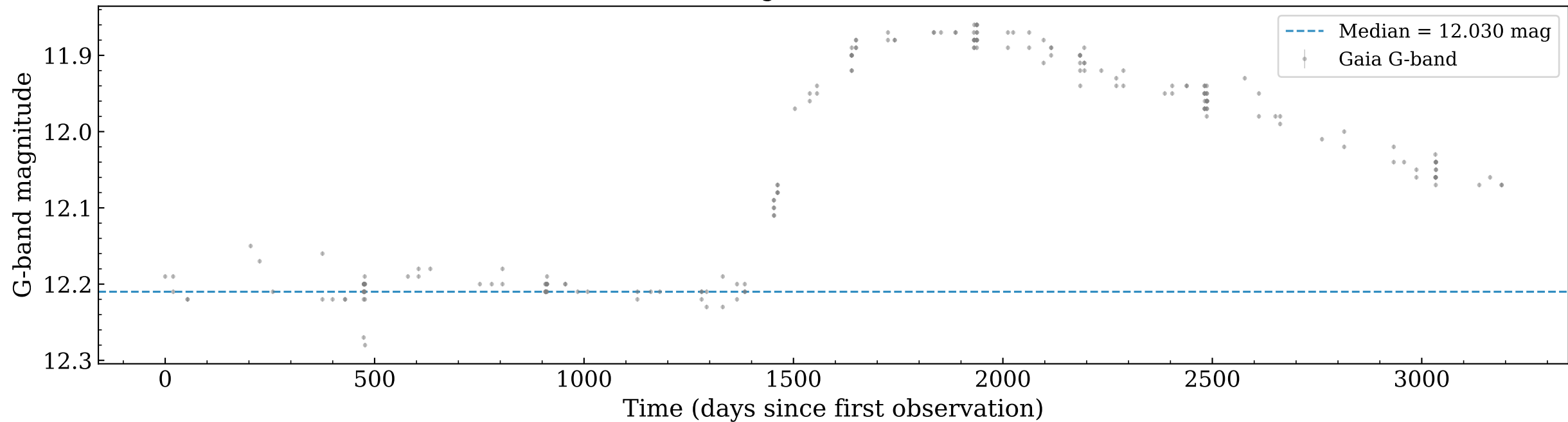
Raw Gaia light curve — Gaia19bzu
